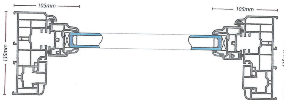
Horizontal section through top sash
