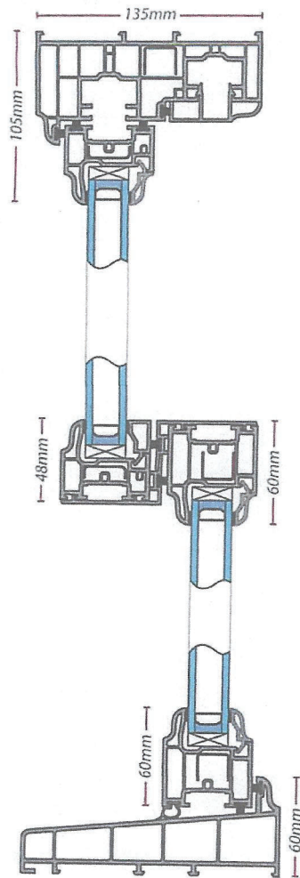
Vertical section through sash with standard sill
