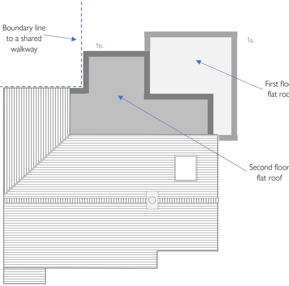
Proposed Roof Layout 1:100
