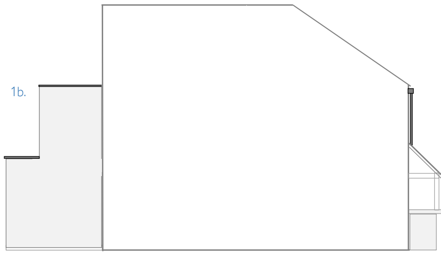
Proposed Southwest Side Elevation 1:100
