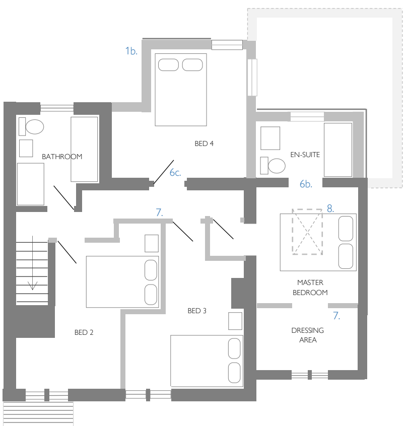
Proposed First Floor Layout 1:100
