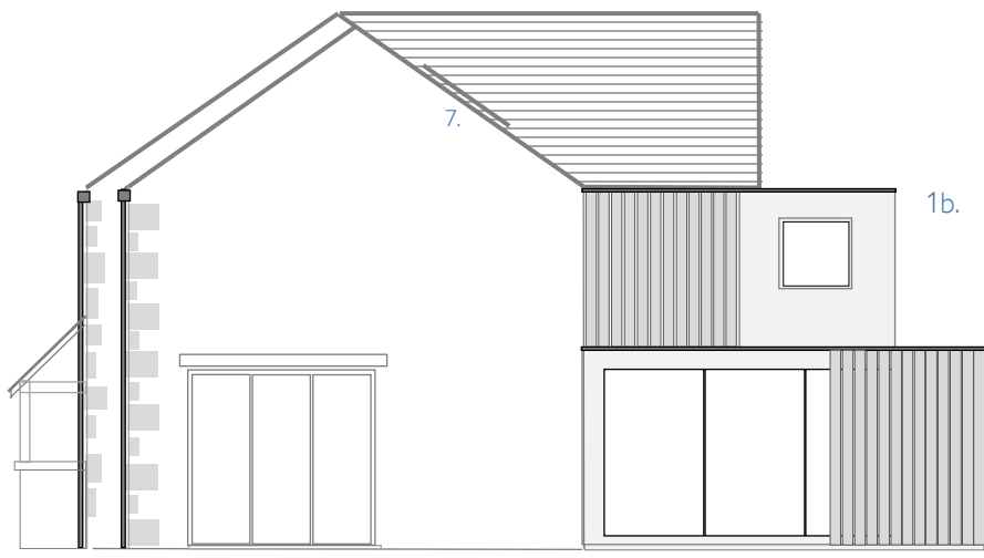
Proposed Northeast Side Elevation 1:100
