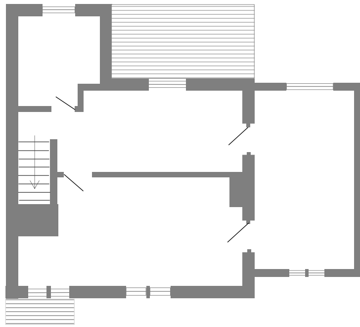
Existing First Floor Layout 1:100
