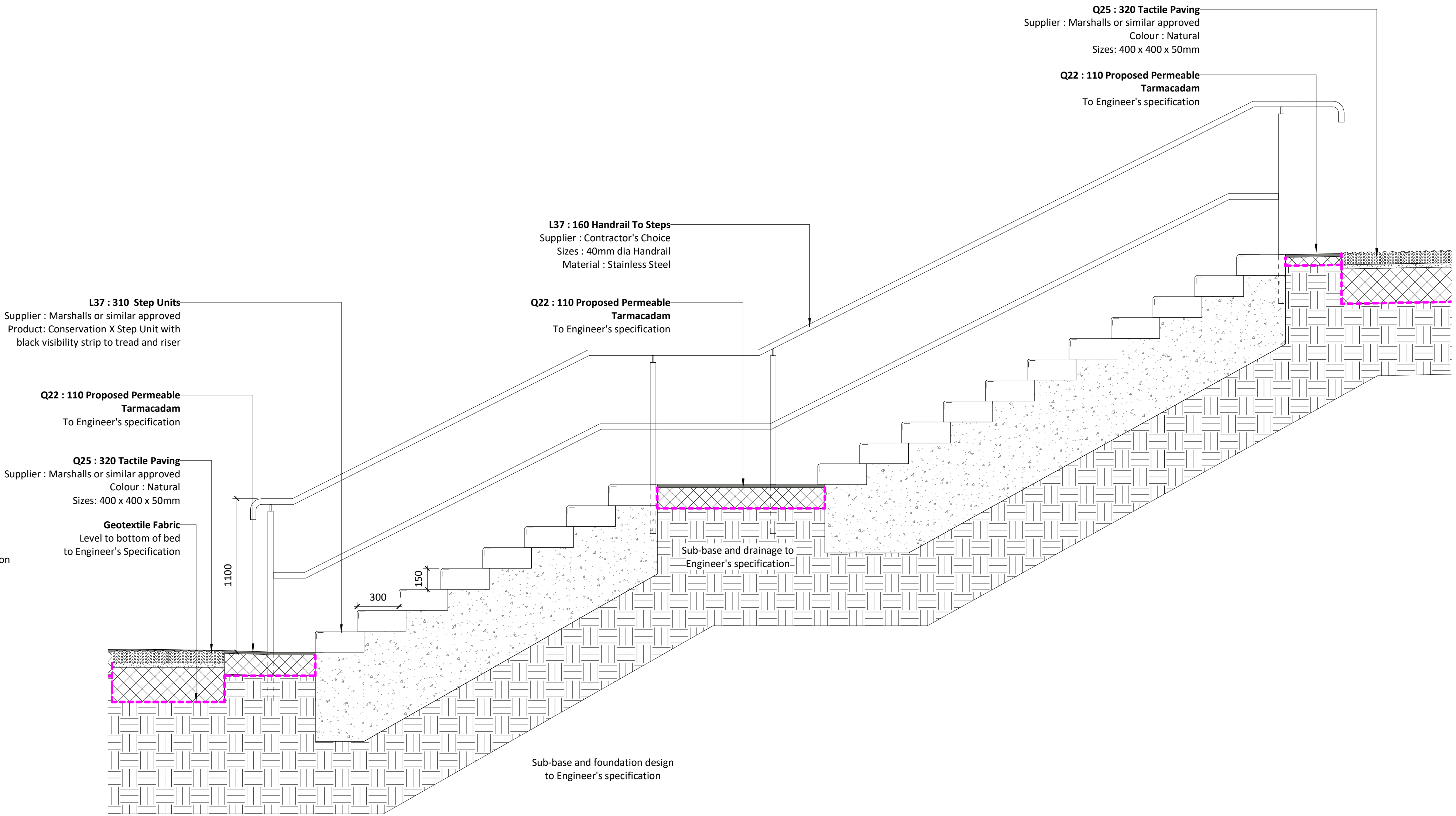
Detail 20 - North West Steps 1 : 20
