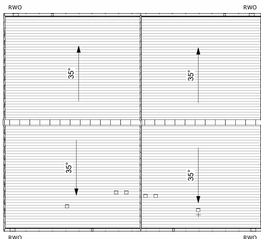
Roof Plan
