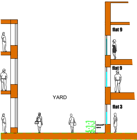
section c-c
