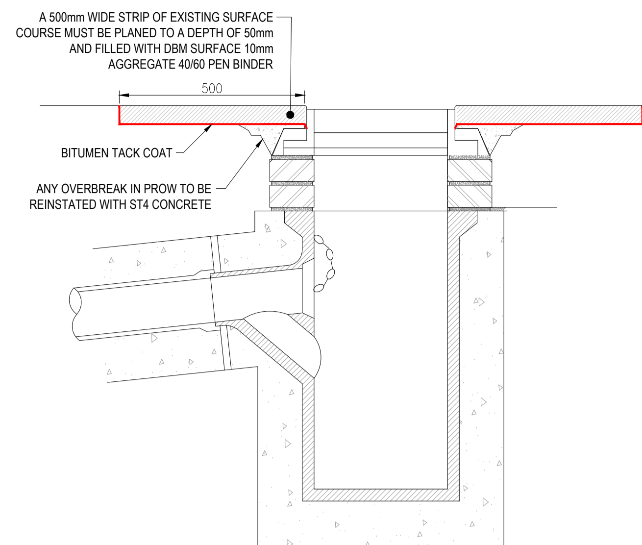
GULLY REINSTATEMENT DETAIL SCALE 1:10
