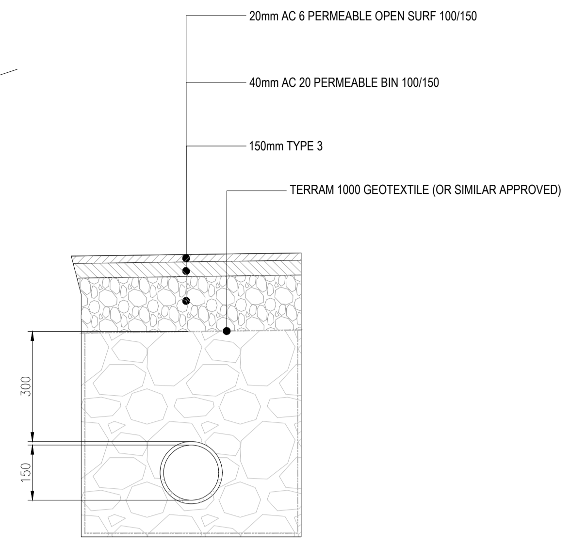
GULLY REINSTATEMENT DETAIL SCALE 1:10
