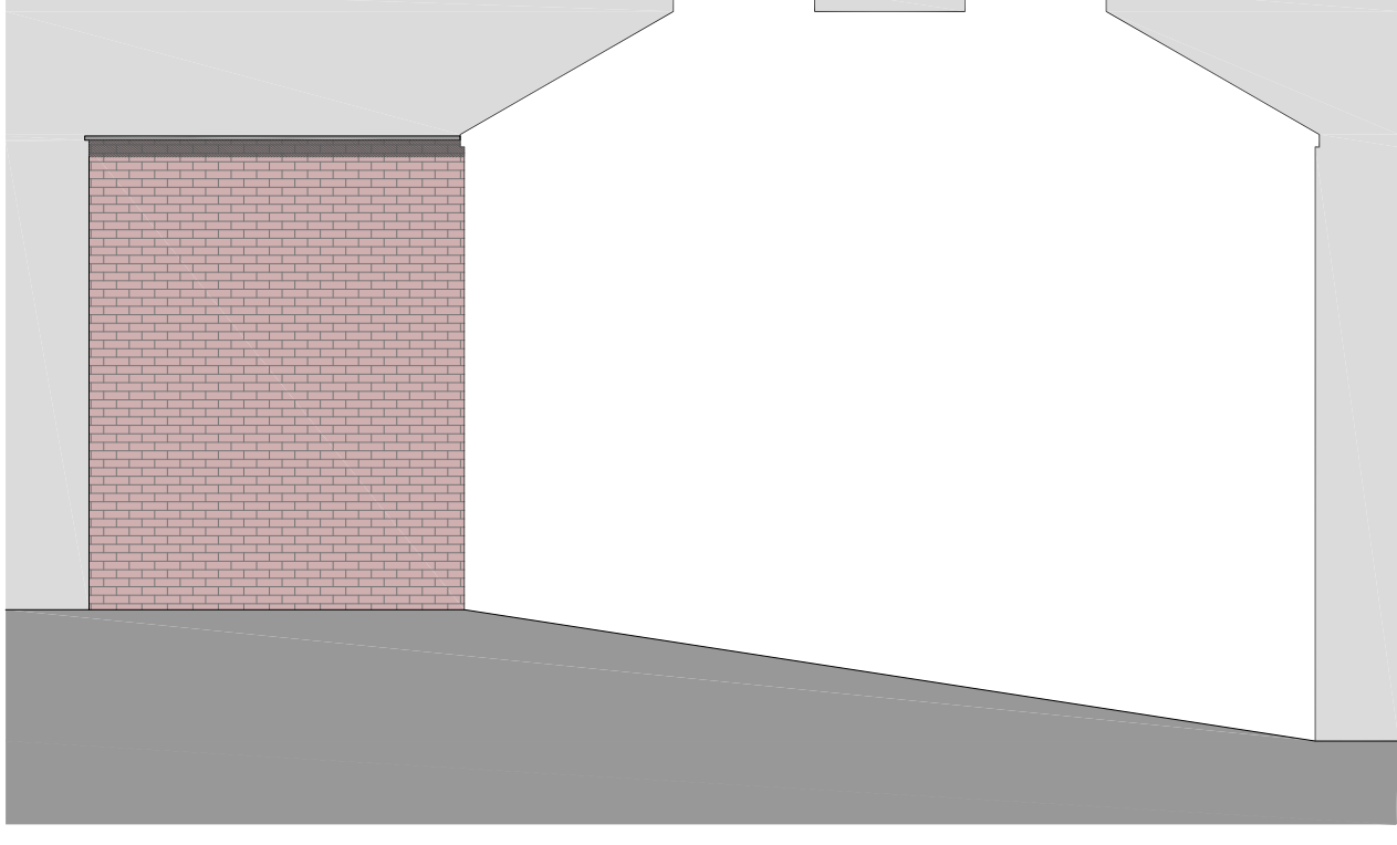
PROPOSED REAR ELEVATION (1:100@A1)
