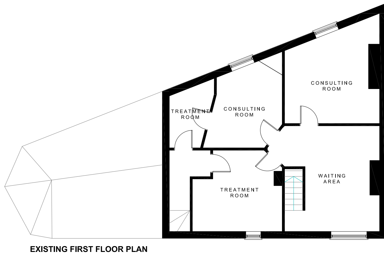
EXISTING FIRST FLOOR PLAN (1:100@A1)
