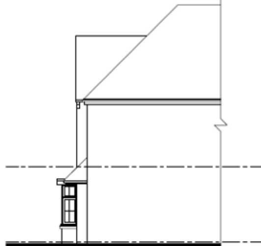
RIGHT SIDE ELEVATION AS PROPOSED (UNCHANGED)
