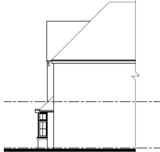
RIGHT SIDE ELEVATION AS EXISTING
