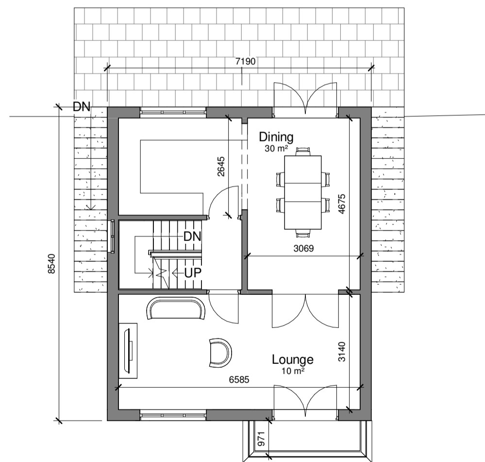
1_First Floor 1 : 100
