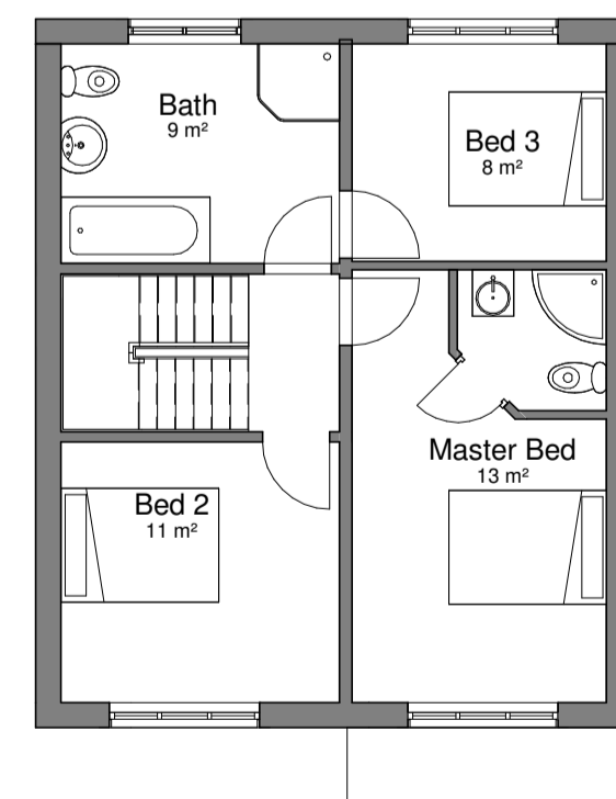
2_Second Floor 1 : 100
