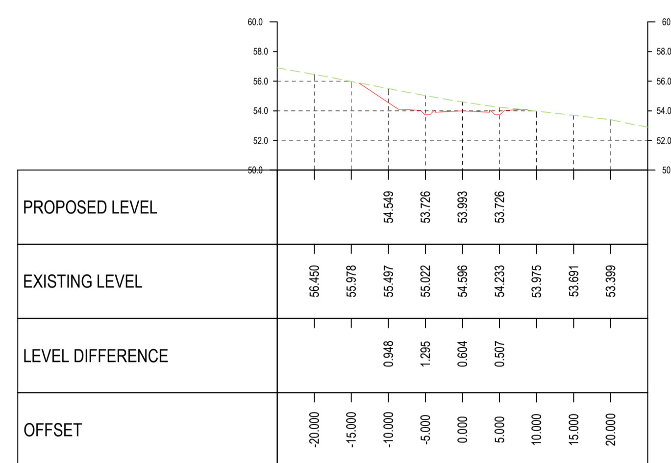
Road 4 Alignment CH 0+200.00 SCALES: H 1:500, V 1:250
