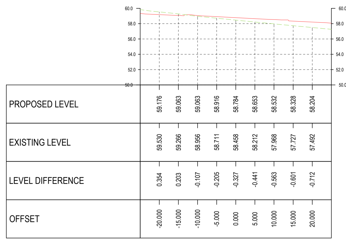
Road 4 Alignment CH 0+000.00 SCALES: H 1:500, V 1:250
