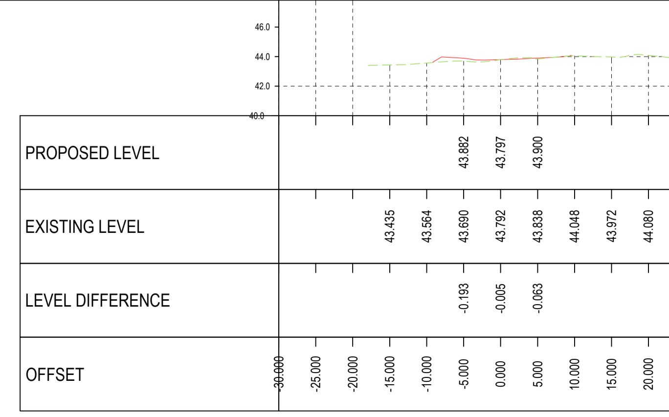
Ex Road 3 Alignment (Rthpe North) CH 0+025.00 SCALES: H 1:500, V 1:250
