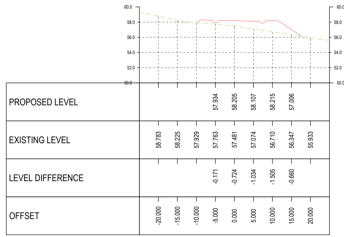
Road 4 Alignment CH 0+050.00 SCALES: H 1:500, V 1:250
