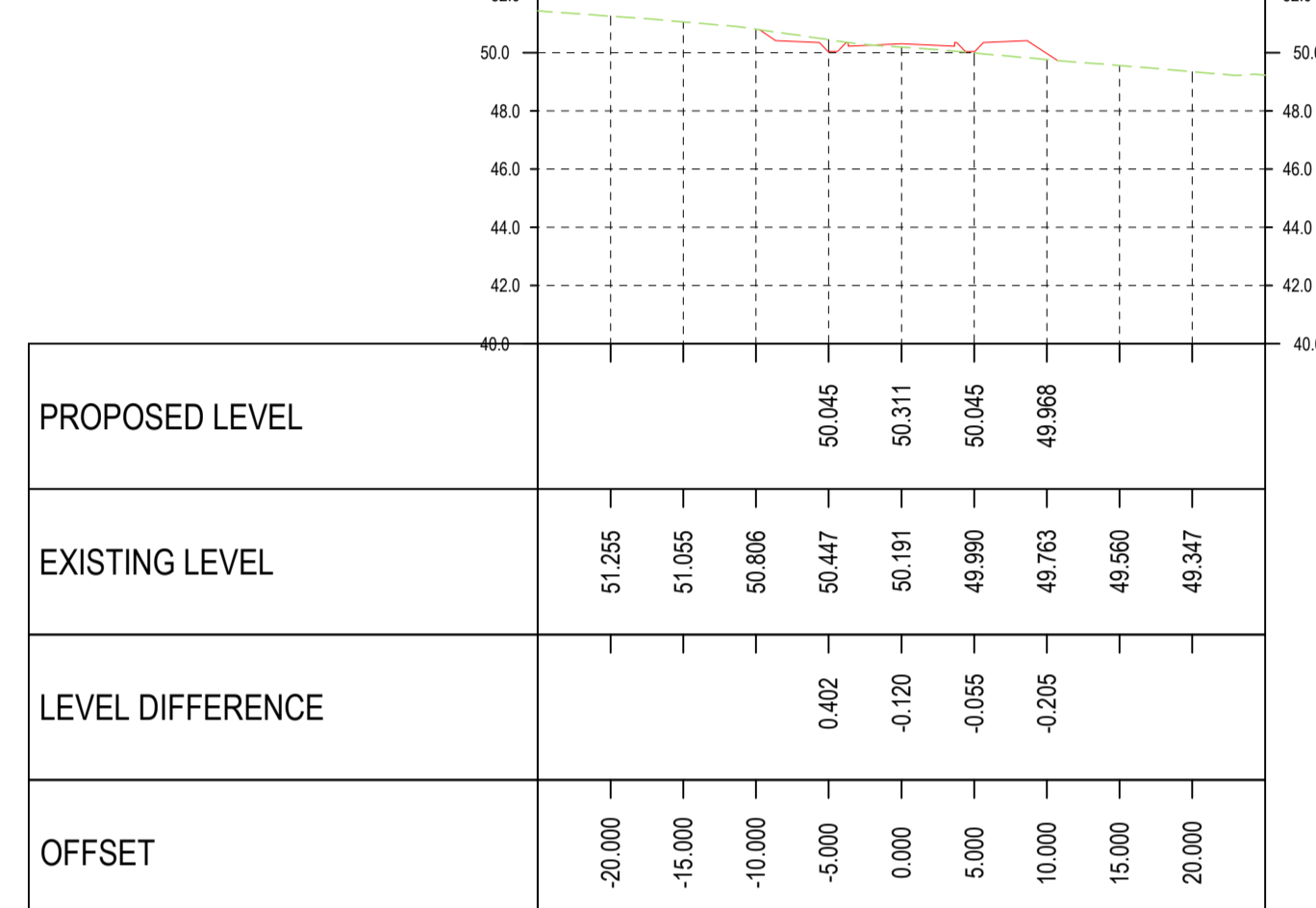
Road 4 Alignment CH 0+400.00 SCALES: H 1:500, V 1:250
