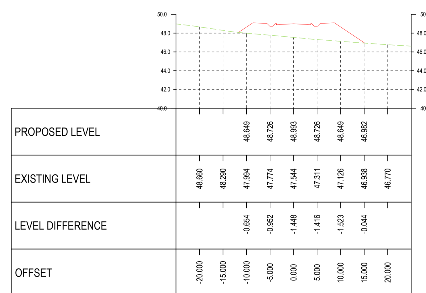
Road 4 Alignment CH 0+300.00 SCALES: H 1:500, V 1:250
