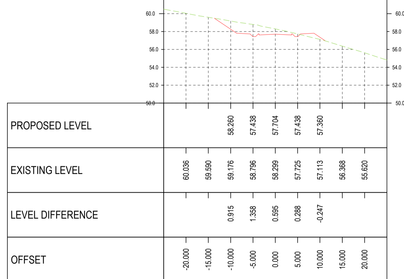
Road 4 Alignment CH 0+100.00 SCALES: H 1:500, V 1:250
