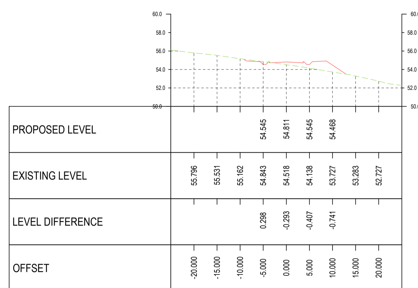
Road 4 Alignment CH 0+500.00 SCALES: H 1:500, V 1:250
