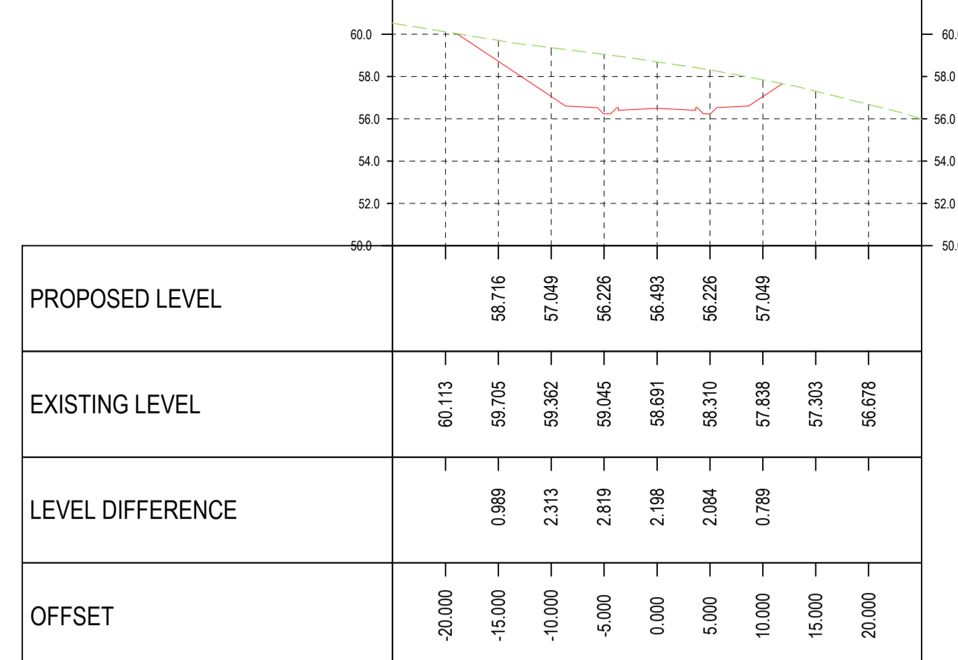
Road 4 Alignment CH 0+150.00 SCALES: H 1:500, V 1:250
