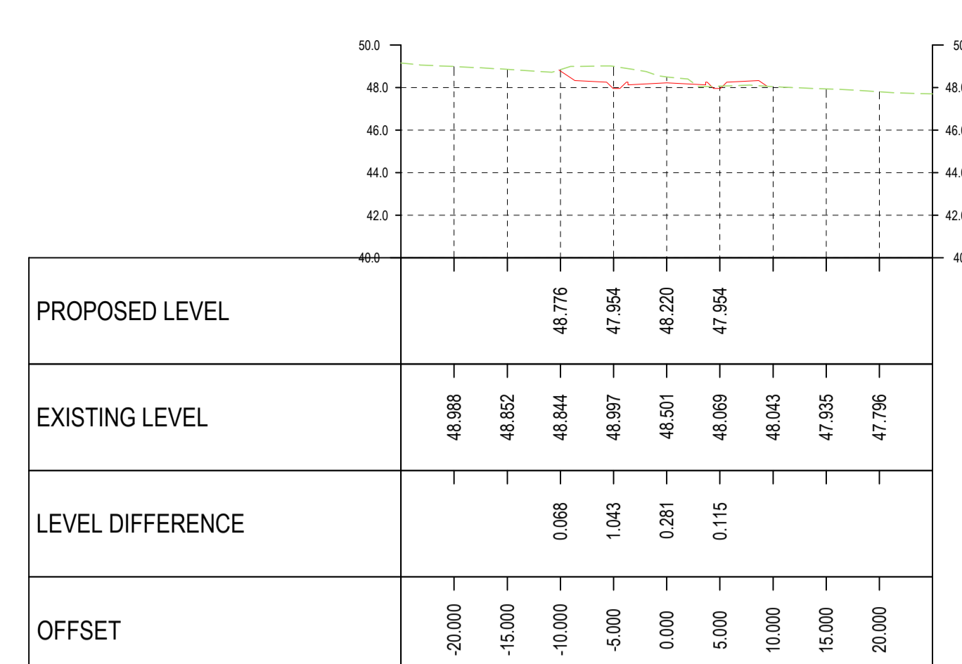
Road 4 Alignment CH 0+350.00 SCALES: H 1:500, V 1:250
