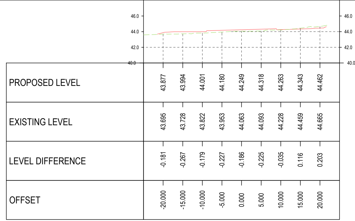
Ex Road 3 Alignment (Rthpe North) CH 0+000.00 SCALES: H 1:500, V 1:250
