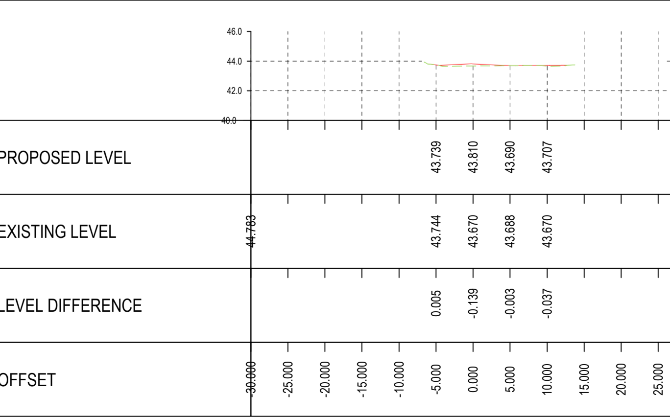
Ex Road 2 Alignment (Rthpe West) CH 0+050.00 SCALES: H 1:500, V 1:250
