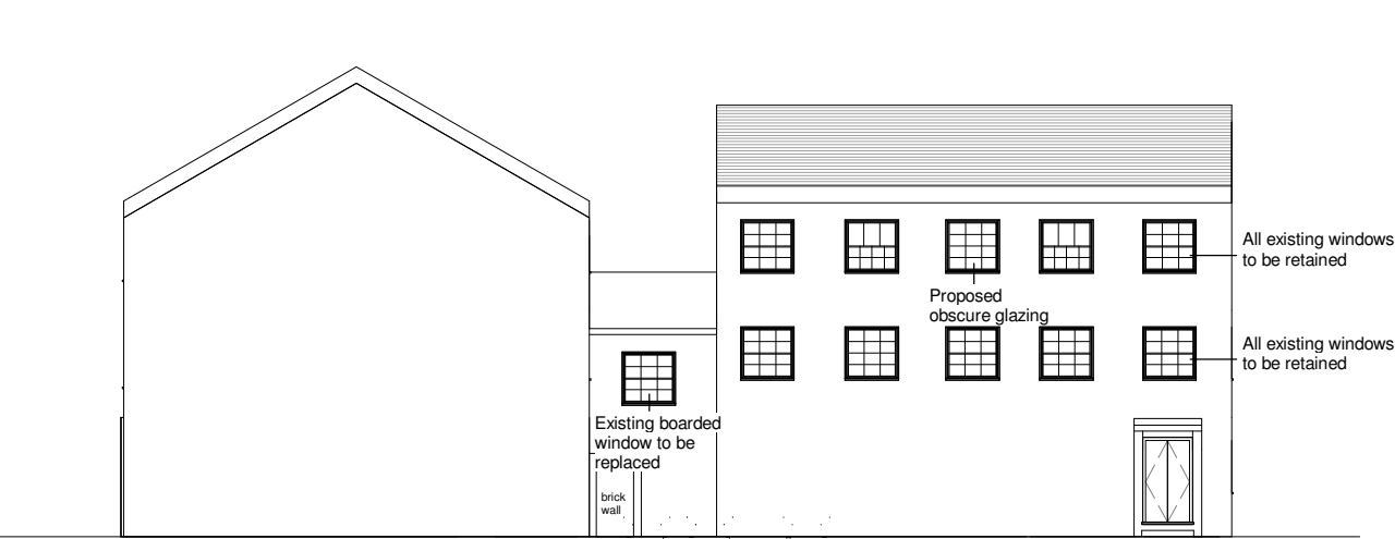
North Elevation
