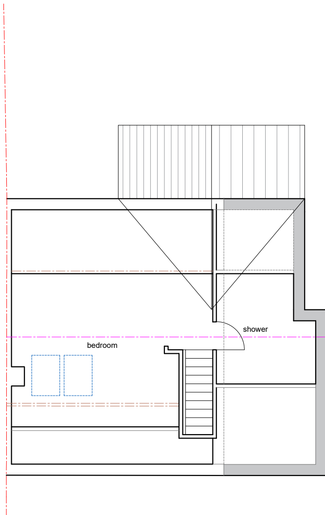
Loft Floor Plan
