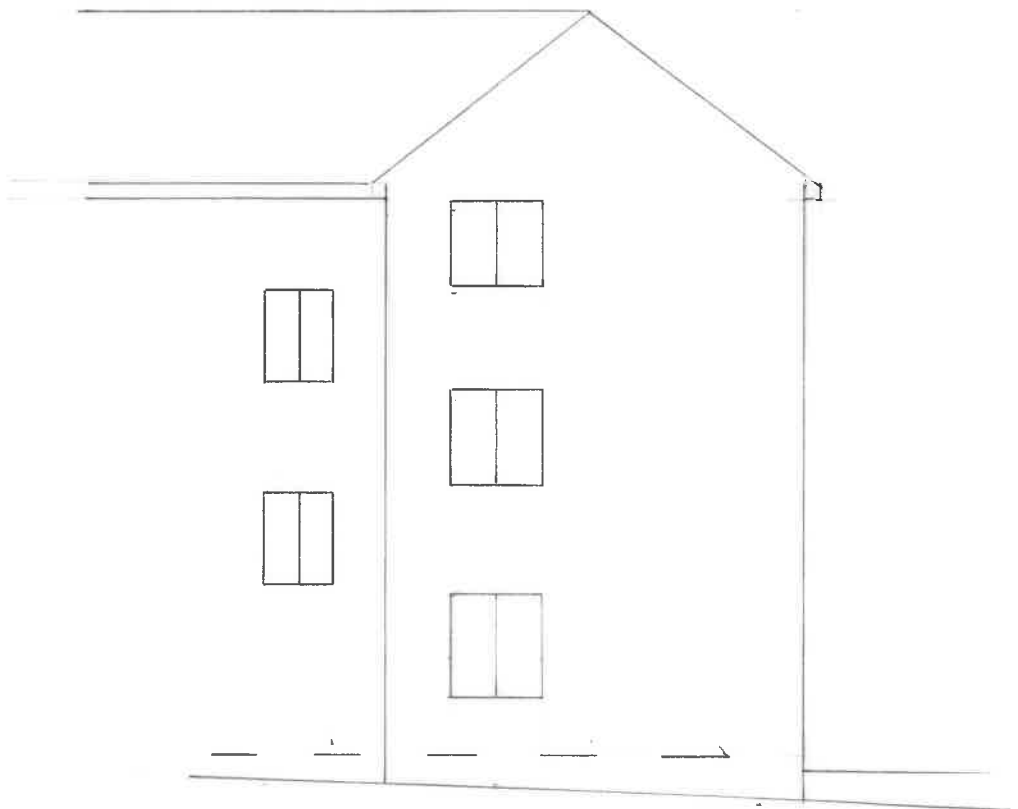
Existing Side
