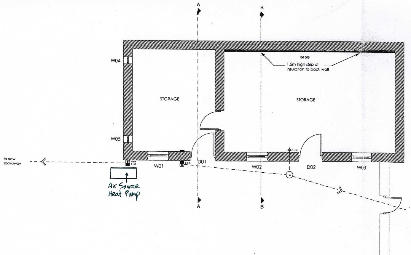
LOWER FLOOR PLAN The Barn, Paddock Farm, Slaithwaite SCALE 1:100
