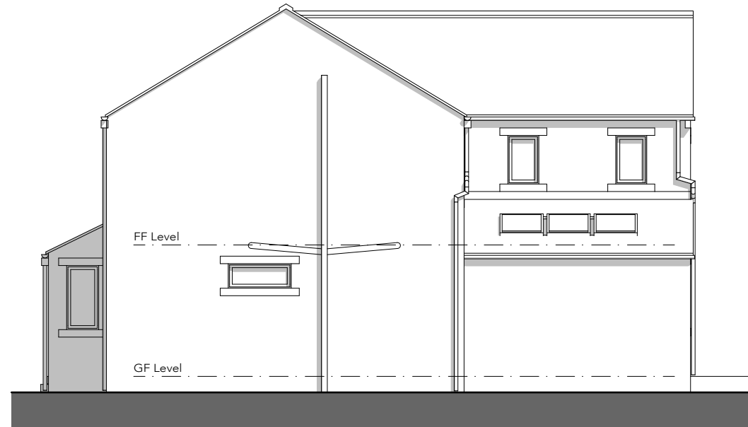
West Elevation 1:100
