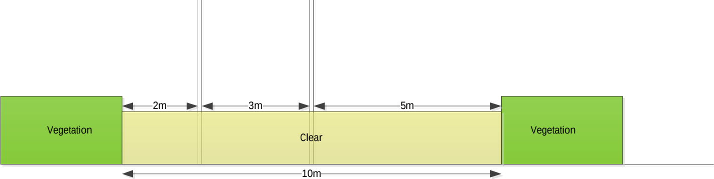
Side View – Pole parallel to vegetation
