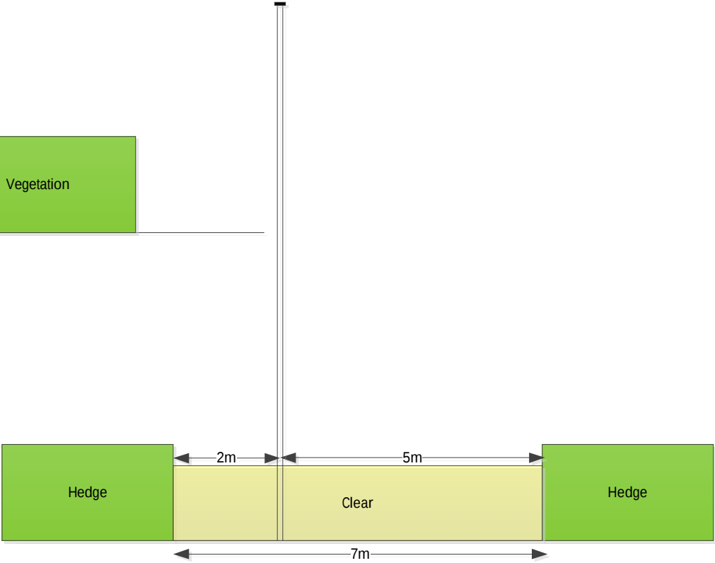
Side View – Pole 90 degrees to hedge
