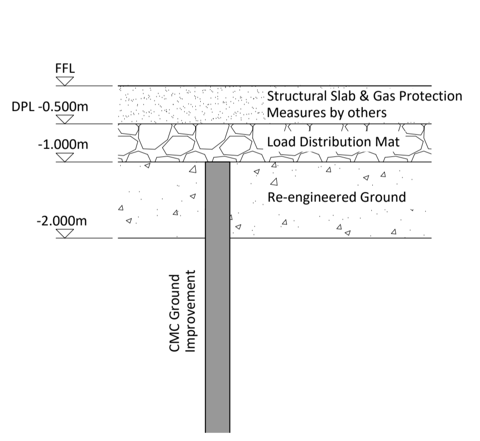
Typical CMC Building Detail Scale 1:50
