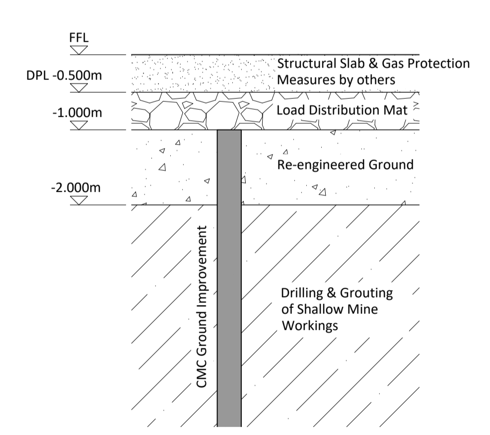
Typical CMC with Mine Workings Building Detail Scale 1:50
