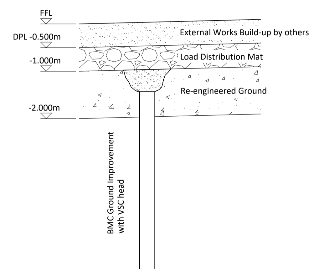
Typical BMC HGV Access Road Detail Scale 1:50
