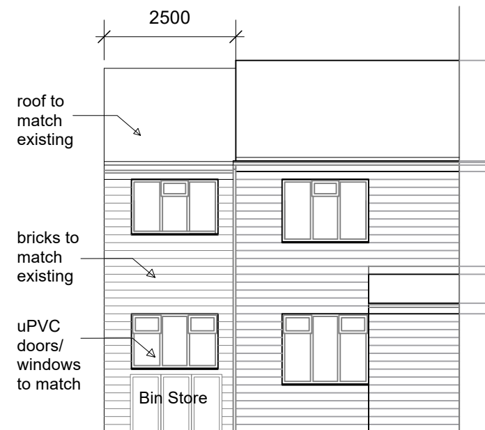
FRONT PROPOSED
