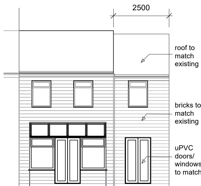
REAR PROPOSED
