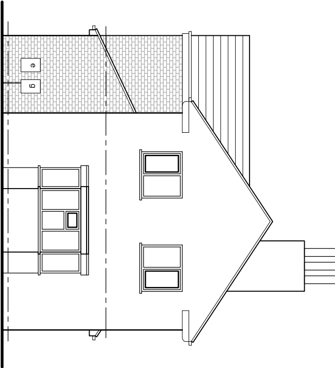
side elevation (facing park)
