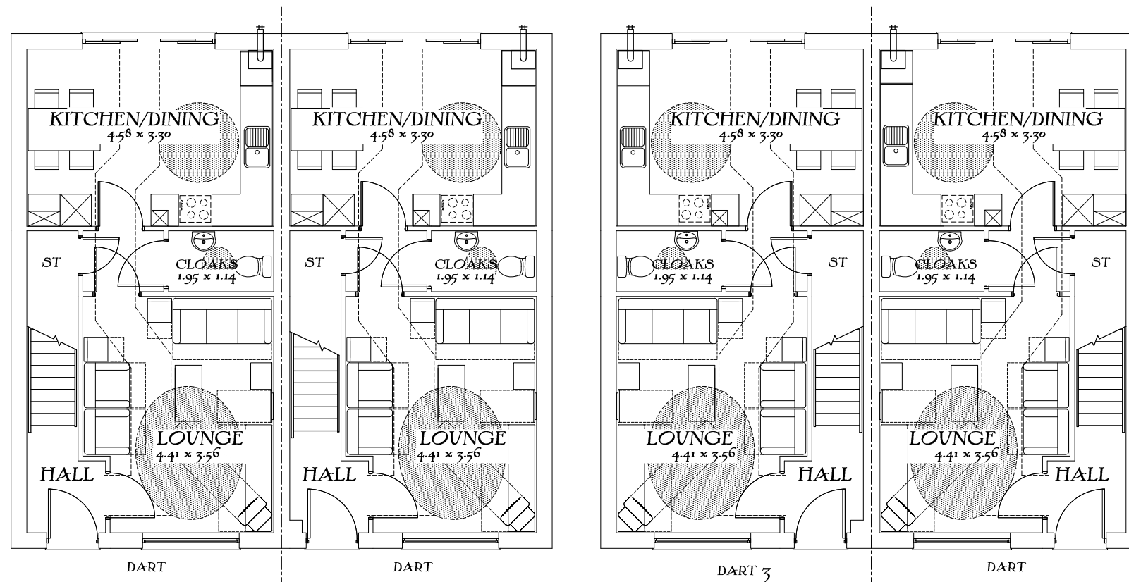
Ground Floor
