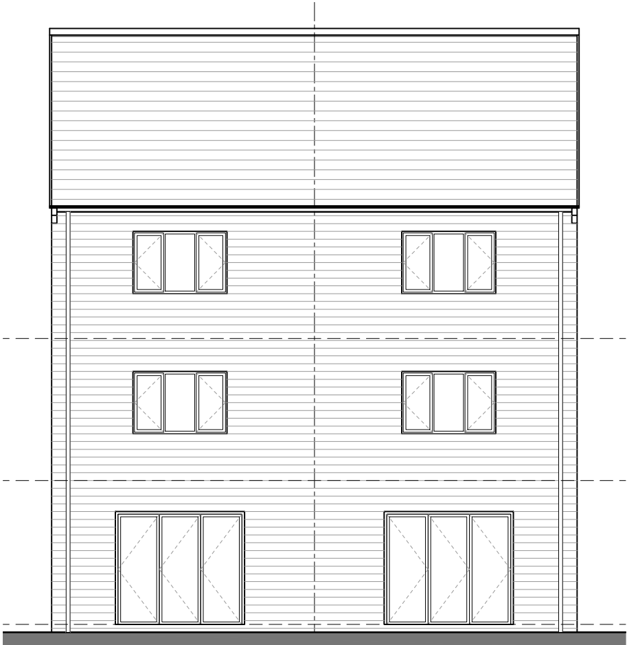
Rear Elevation
