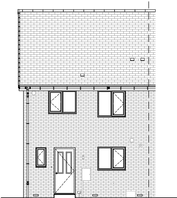
Front Elevation
