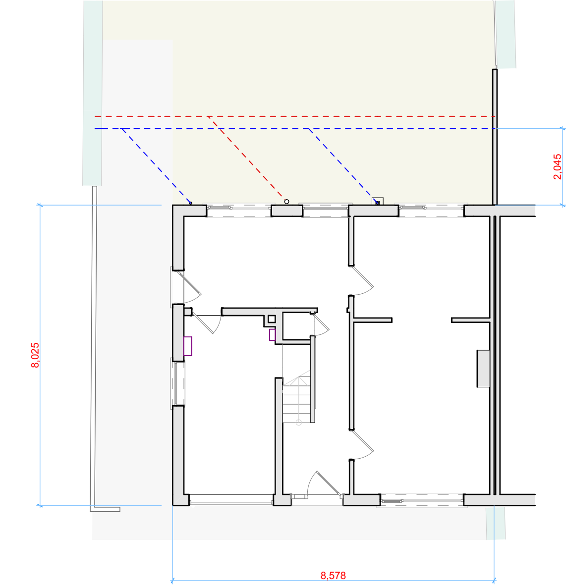
3 Existing Ground Floor 1:100
