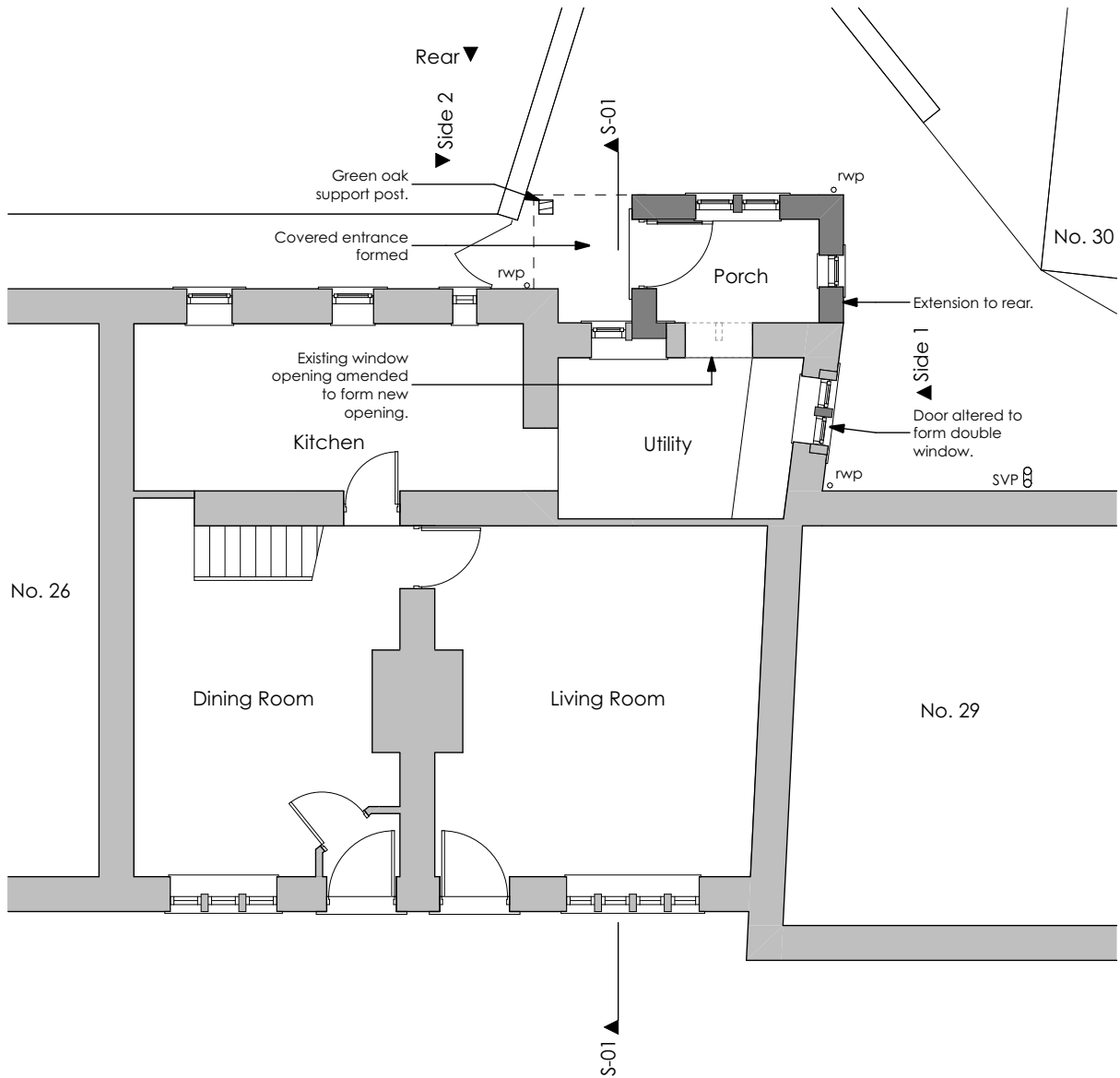
Ground Floor 1:100
