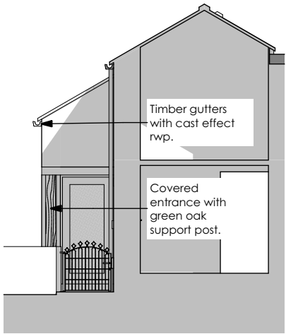
Side 2 Elevation 1:100
