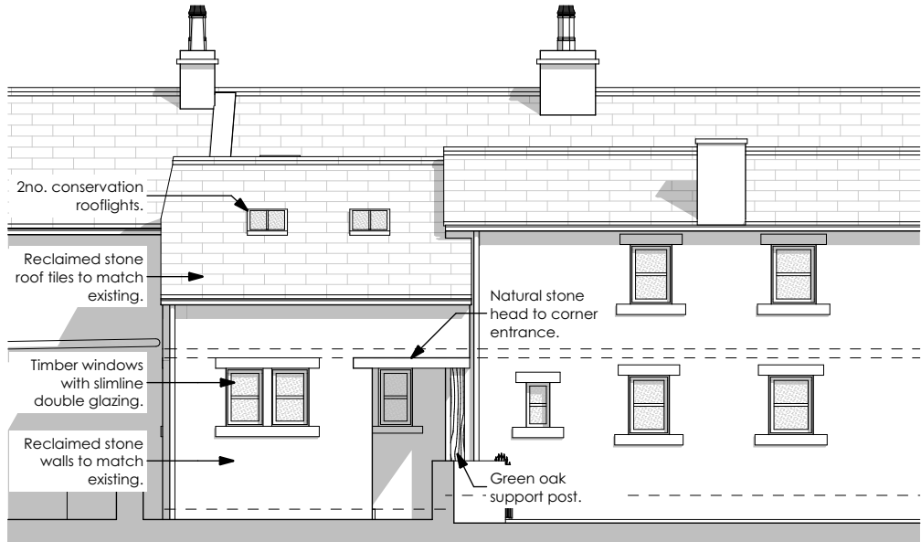
Rear Elevation 1:100
