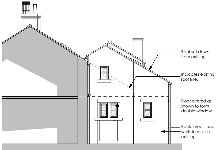
Side 1 Elevation 1:100
