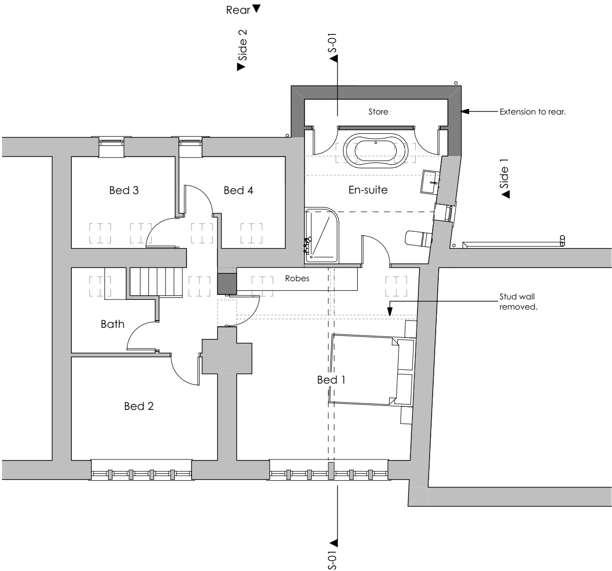
First Floor 1:100
