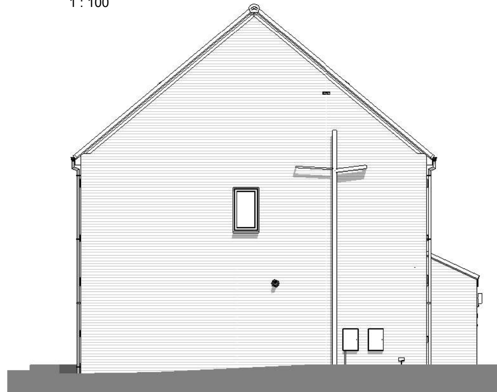
Left Side Elevation 1 : 100
