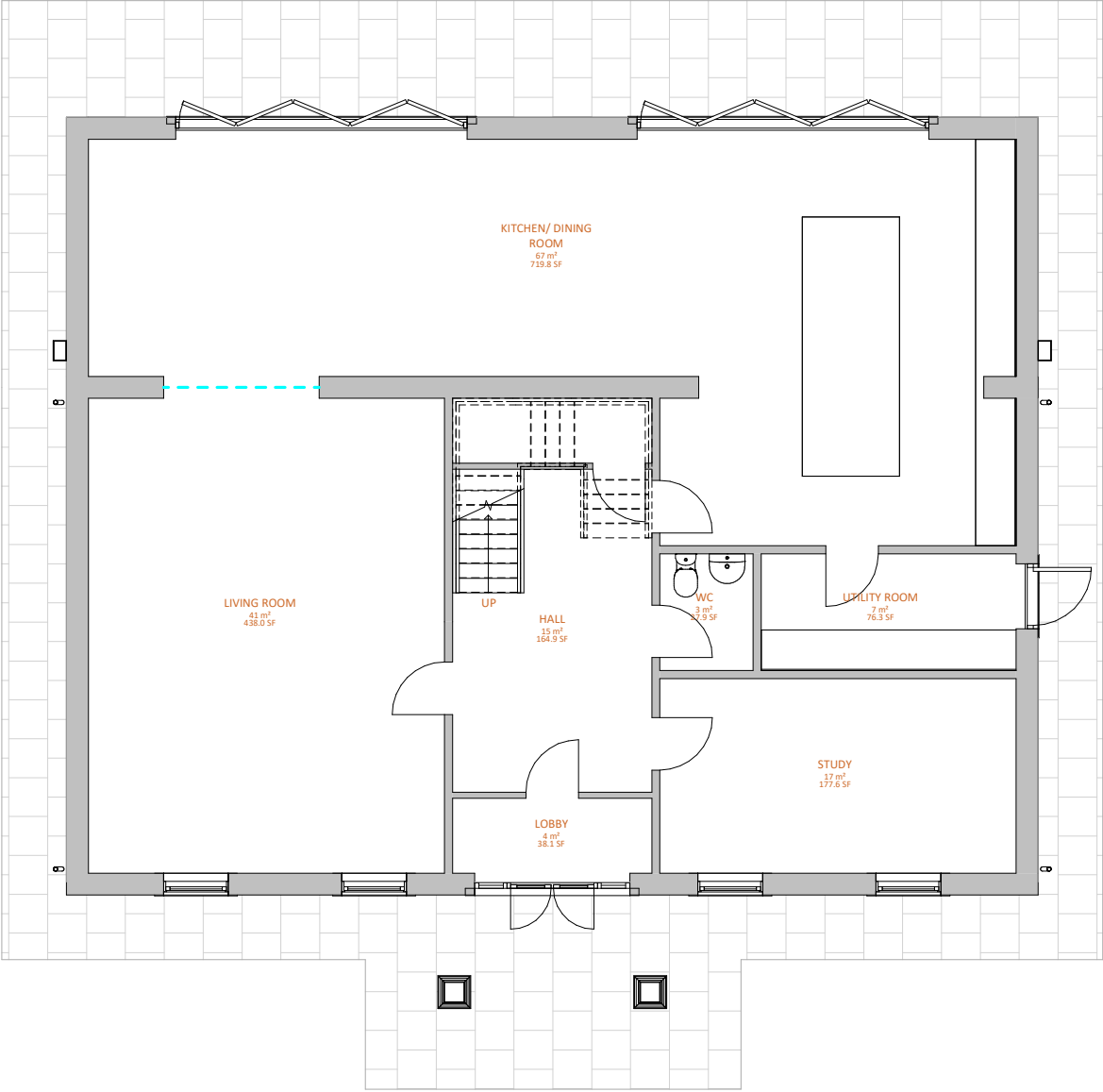
1 Ground Floor Scale - 1 : 50
