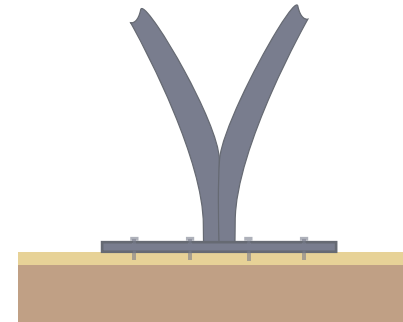
Surface fixing on concrete
