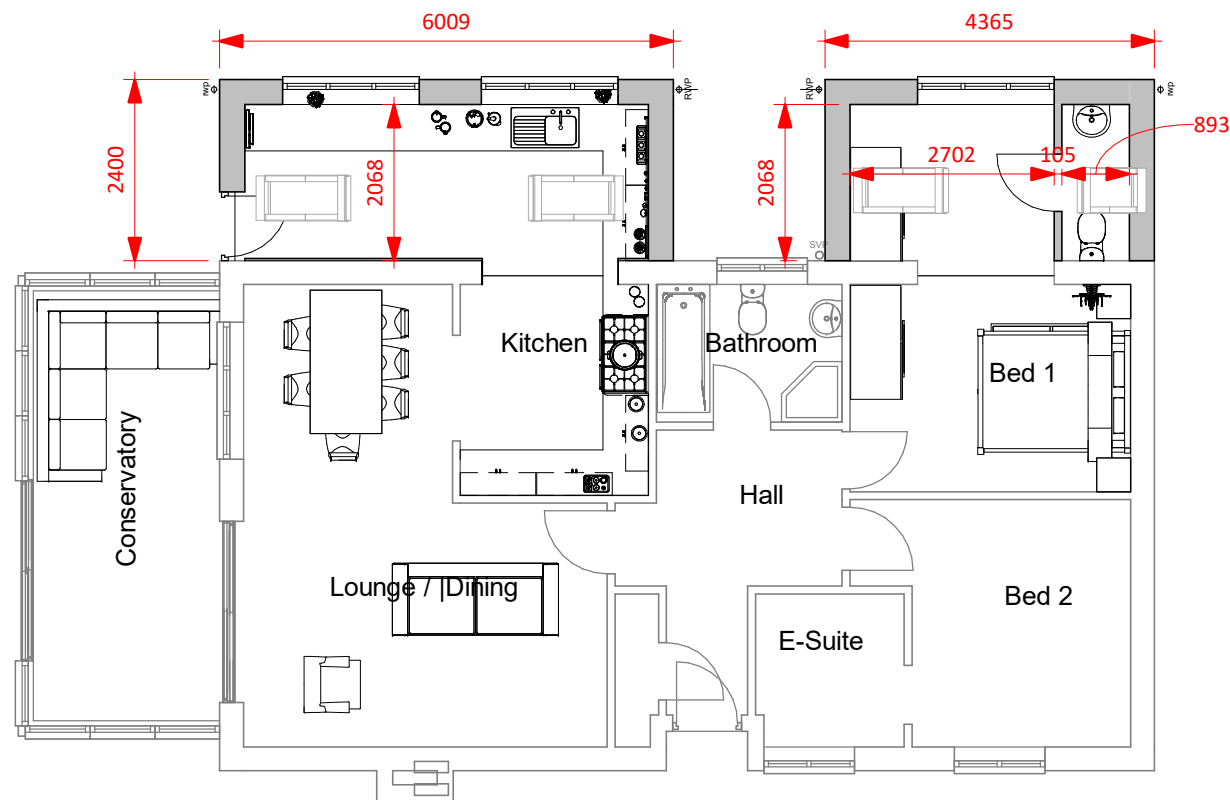
02b GF Proposed 1 : 100
