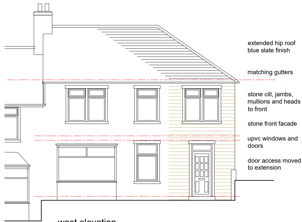
west elevation
