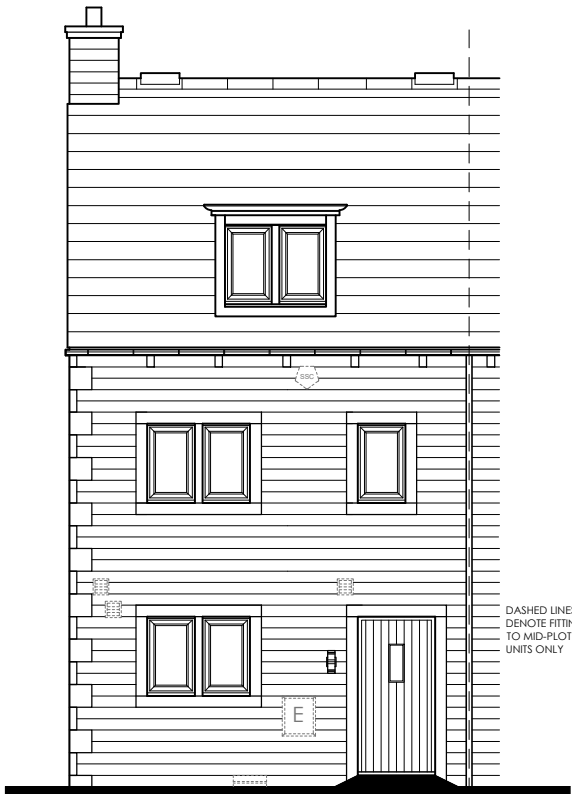
FRONT ELEVATION
