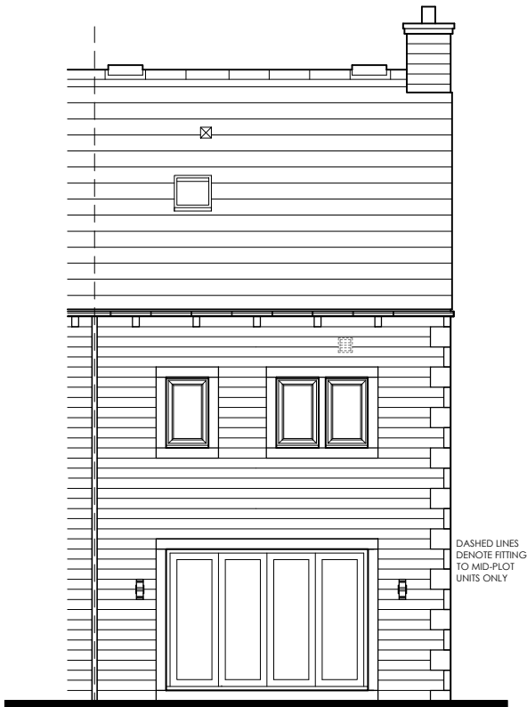
REAR ELEVATION
