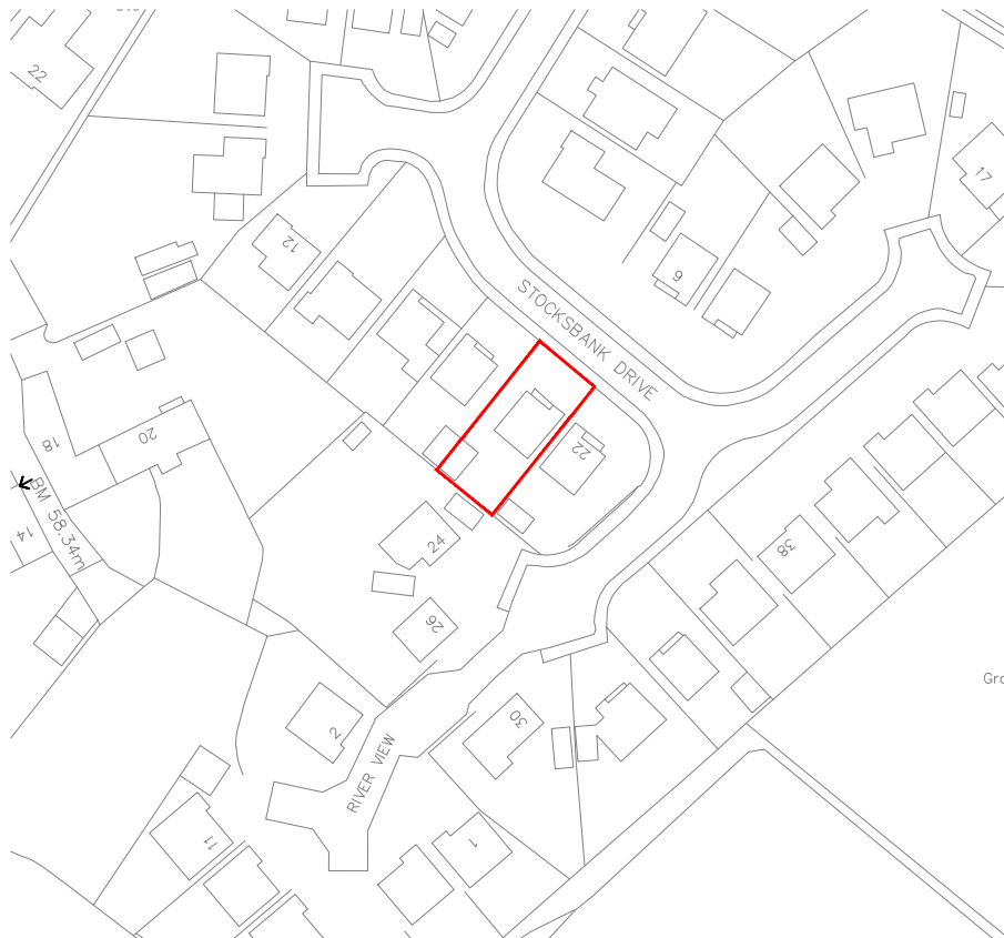
LOCATION PLAN 1:1250
