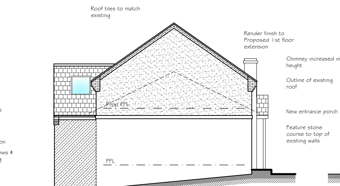
East/Side Elevation As Proposed
