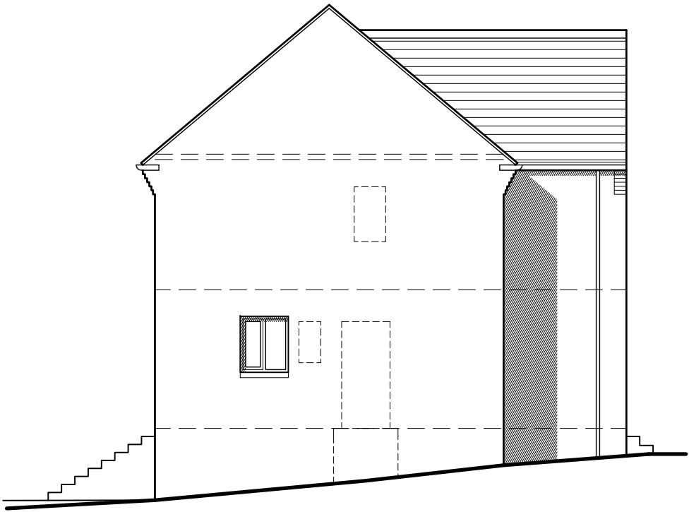
Side Elevation
