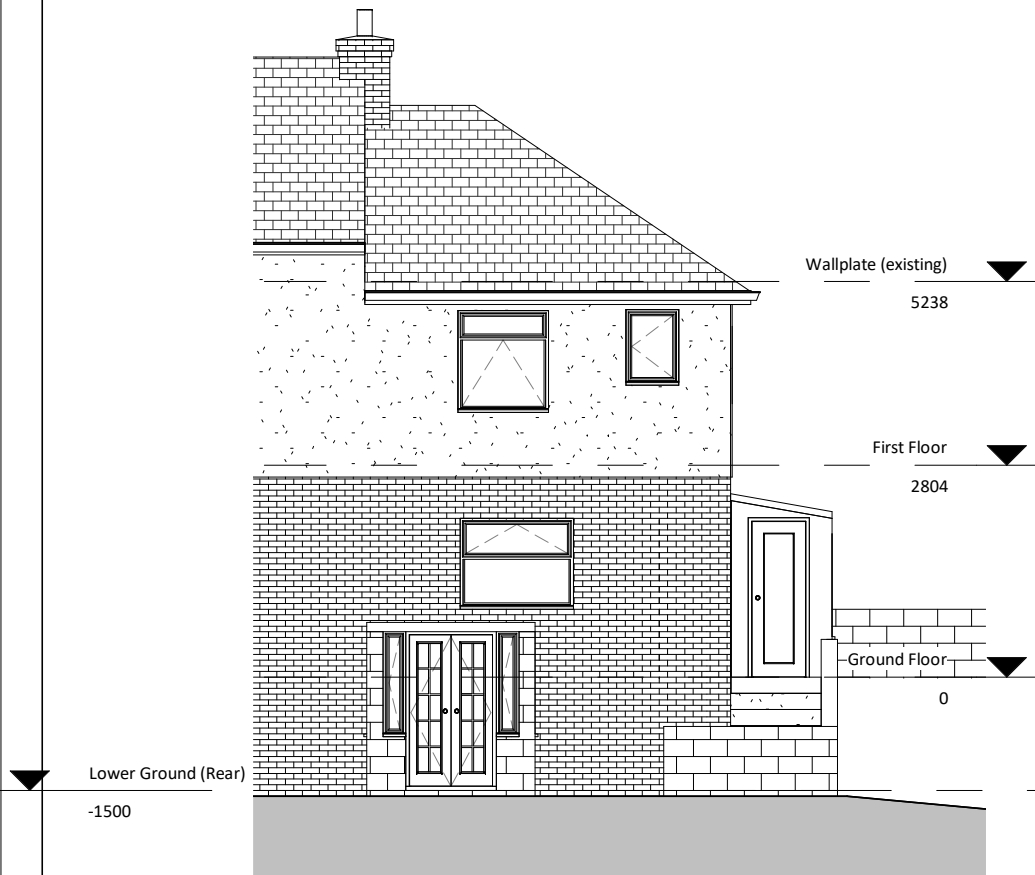
10 Rear Existing 1 : 100
