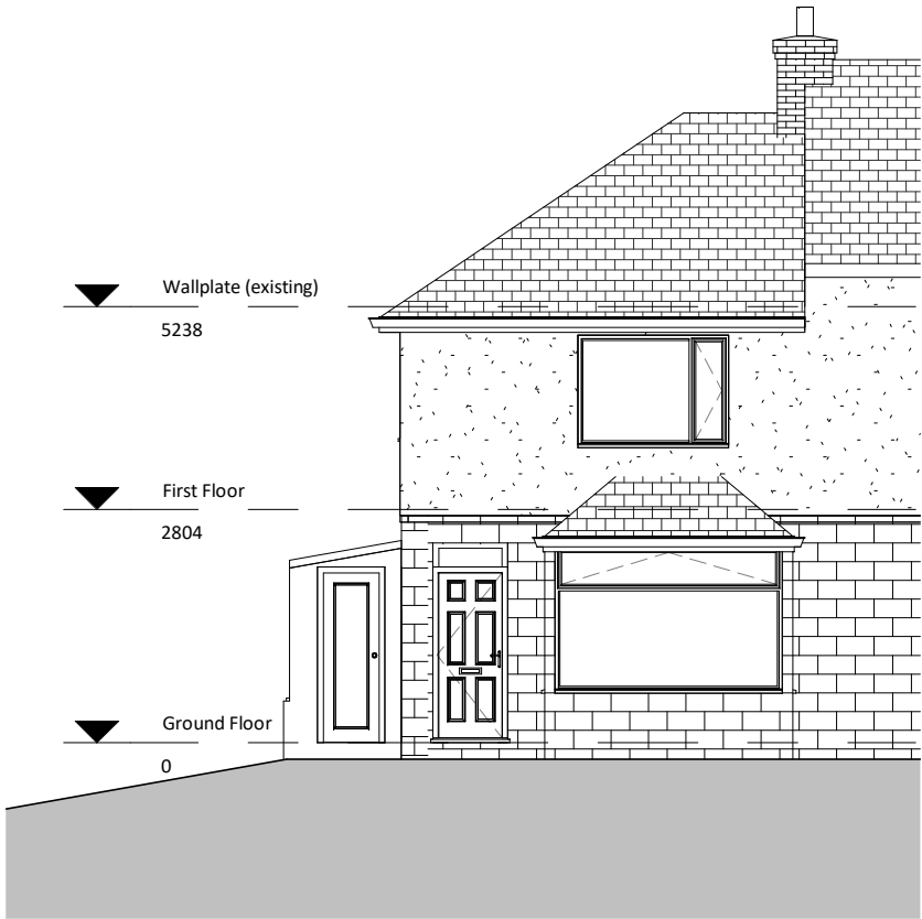
10 Front Existing 1 : 100
