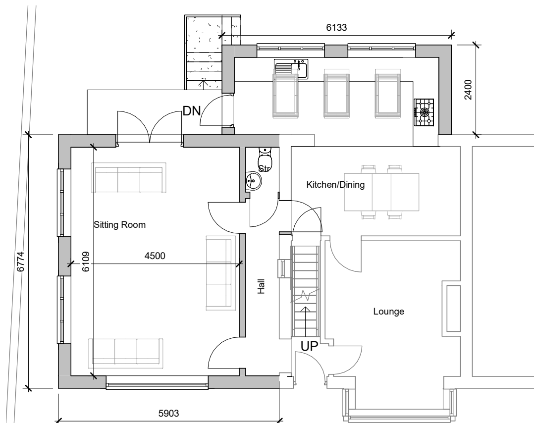
02a GF Proposed 1 : 100
