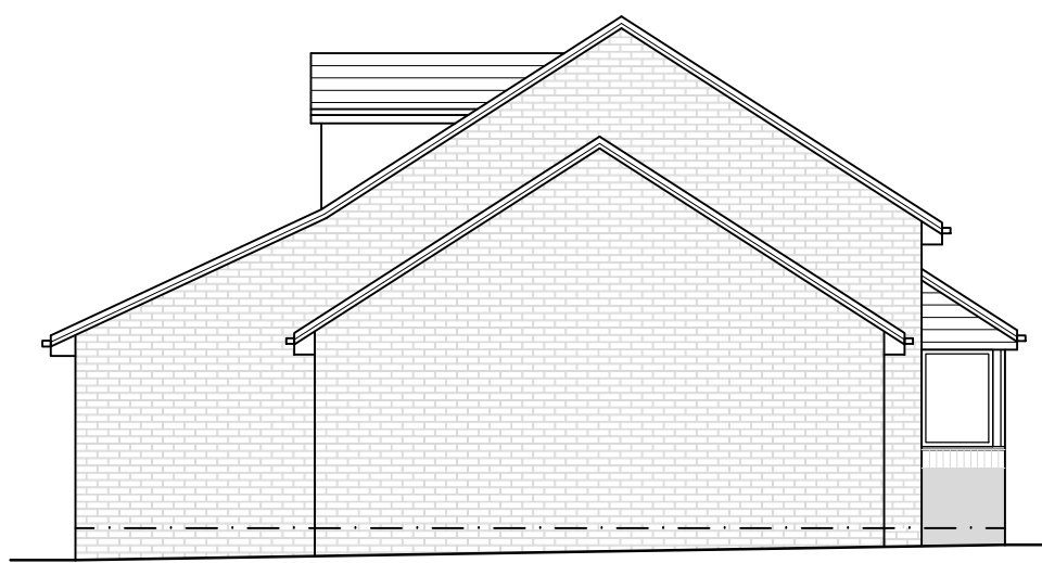
Side Elevation (Garage)
