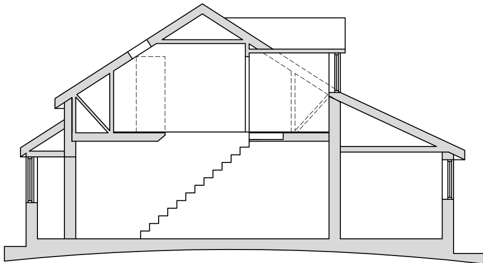
General Section
