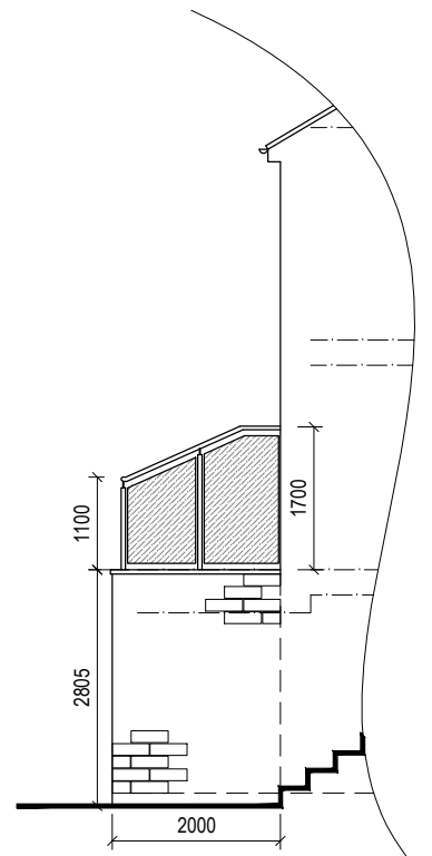
East Elevation
