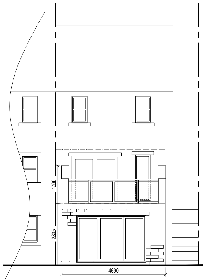
Rear Elevation
