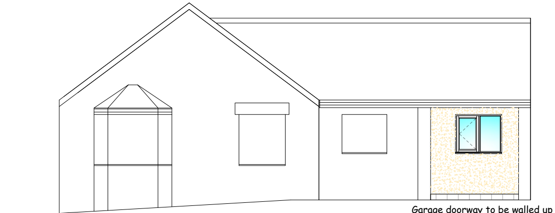
North Elevation
