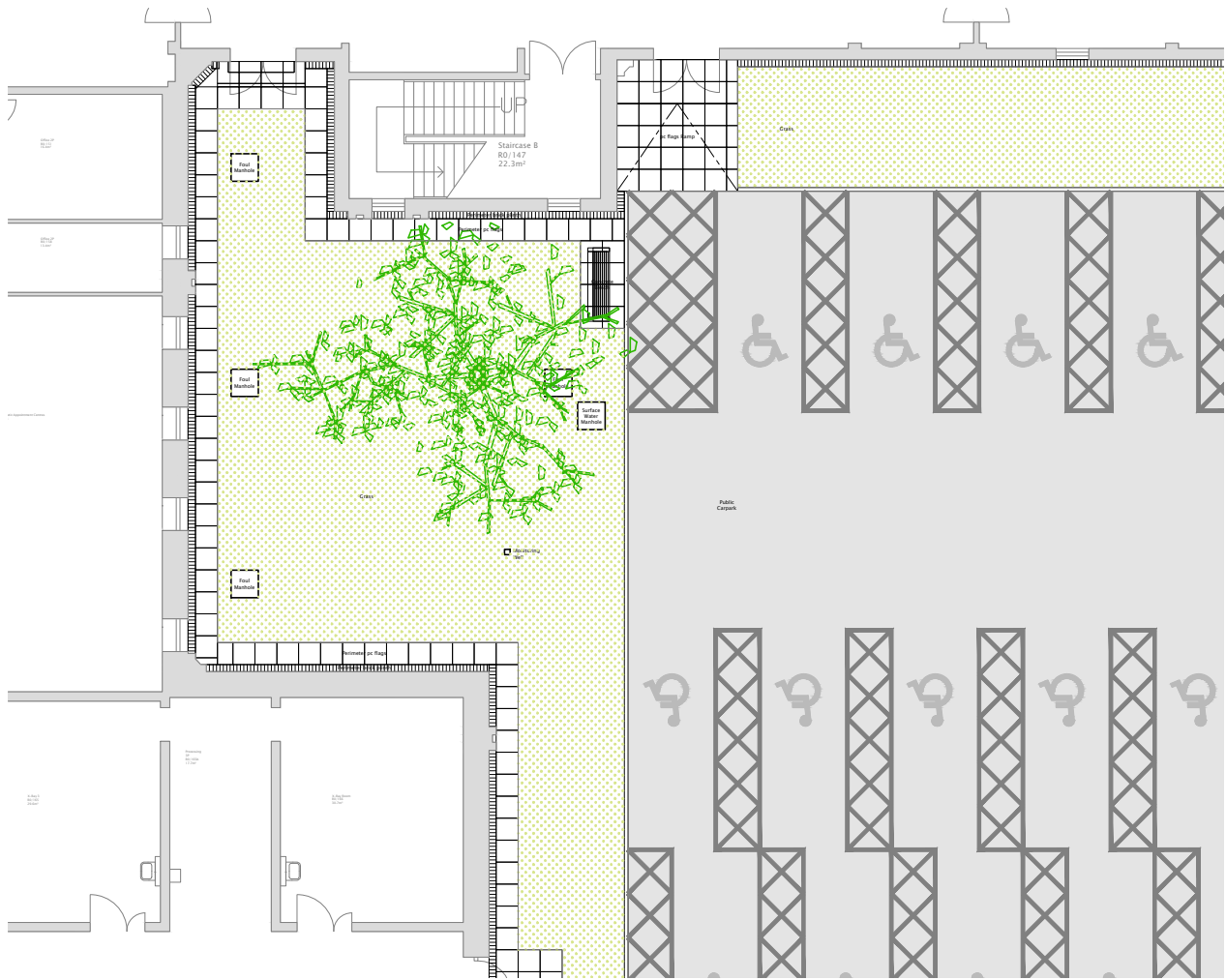
Key Plan as Existing Scale 1:200
