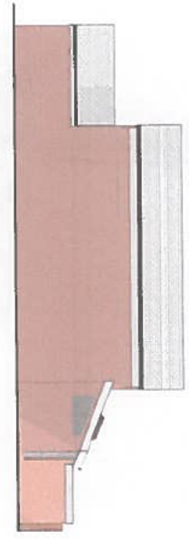
Rear Elevation W 1 : 100
