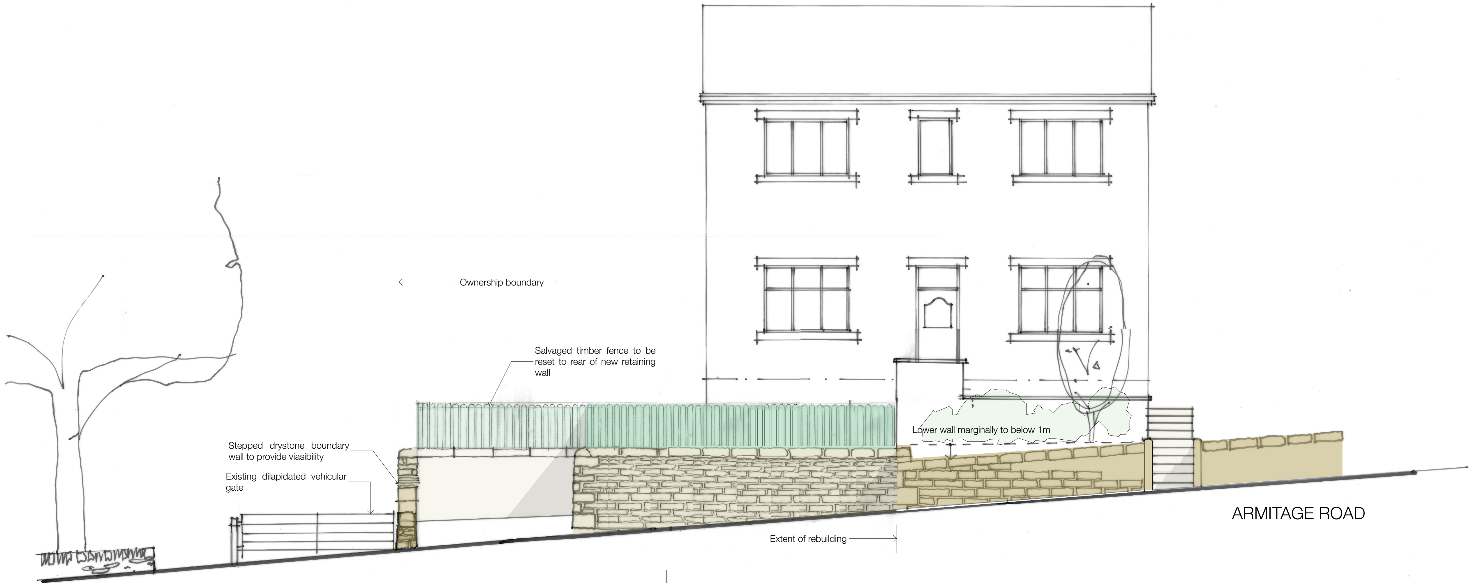
Elevation as Proposed 1:50
