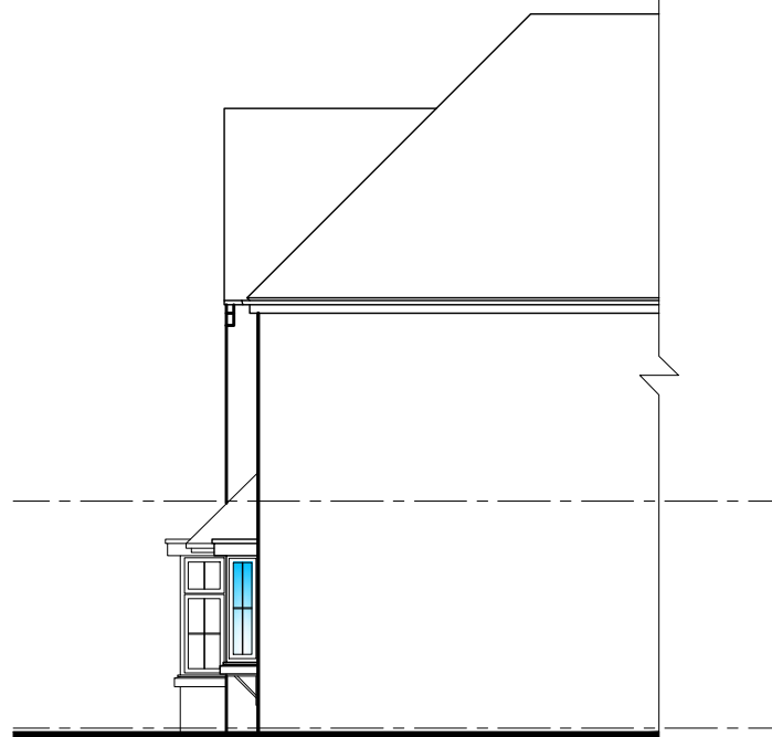
RIGHT SIDE ELEVATION AS PROPOSED
