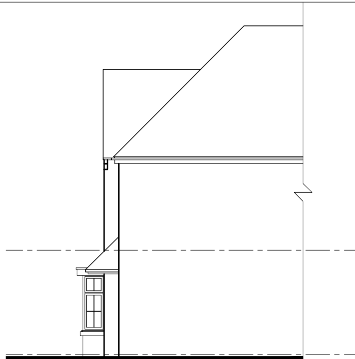
RIGHT SIDE ELEVATION AS EXISTING
