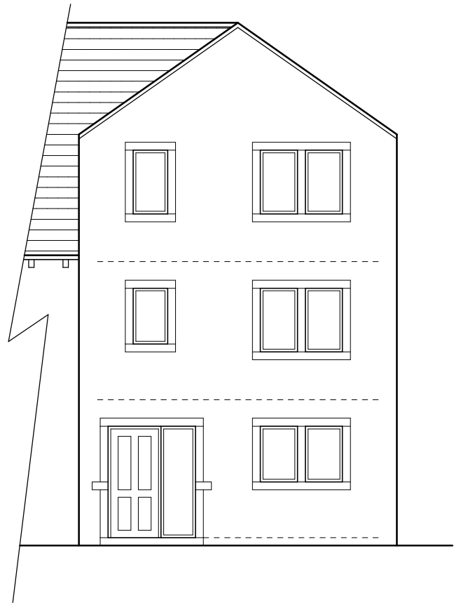
Front elevation (1:100)
