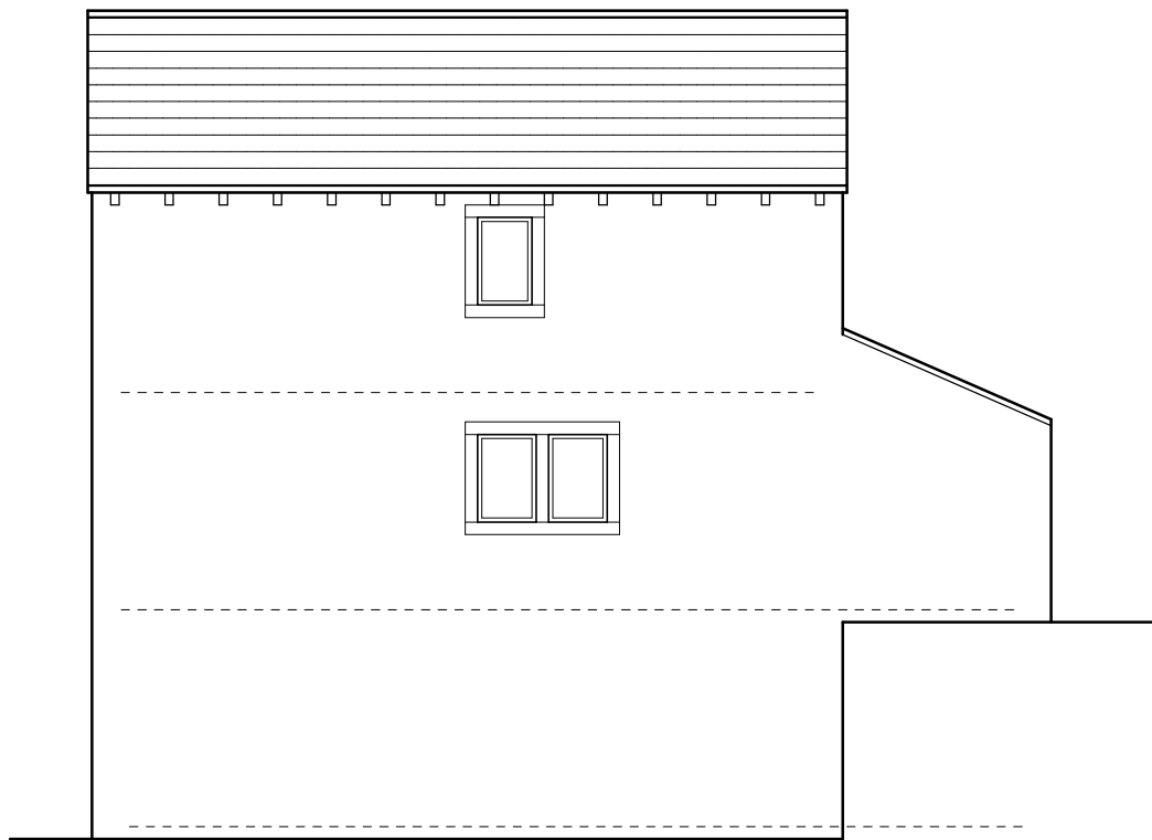
Side elevation (1:100)
