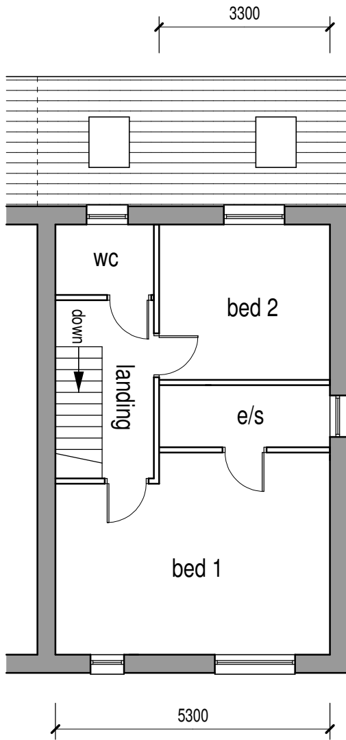
Second Floor (1:100)
