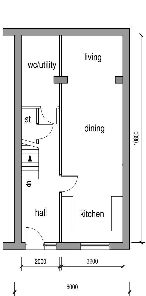
Ground Floor (1:100)
