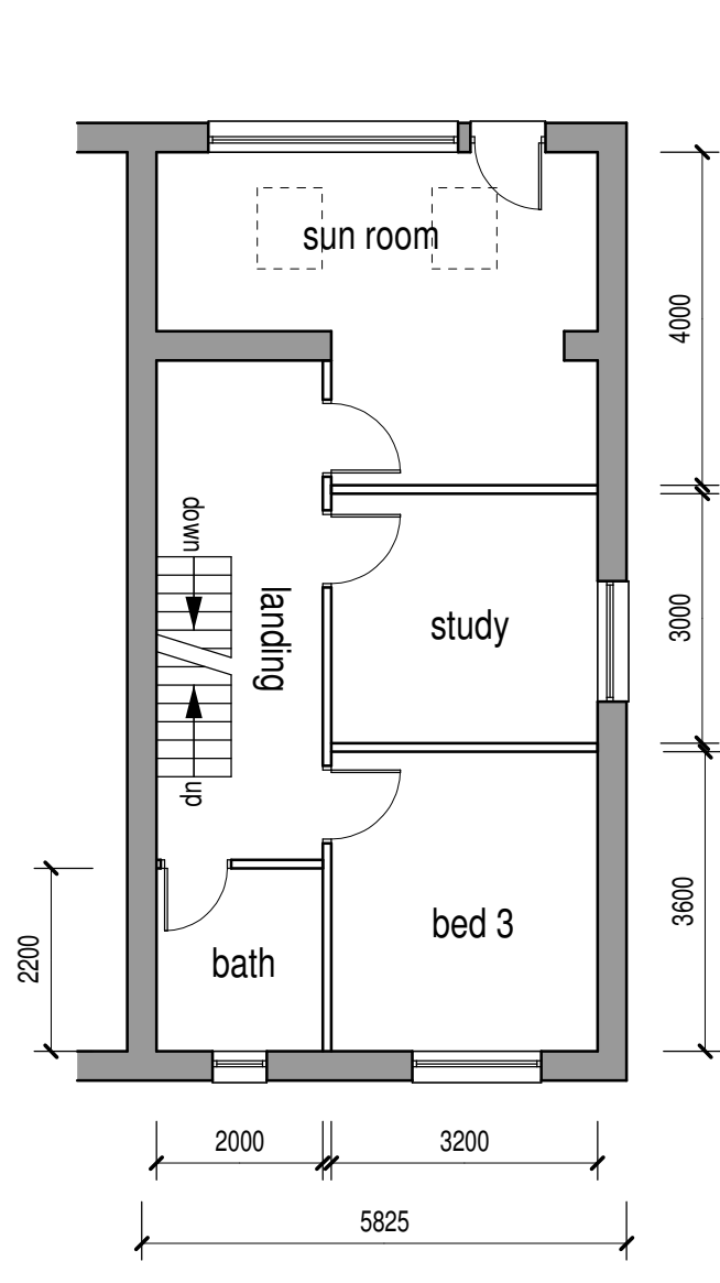
First Floor (1:100)
