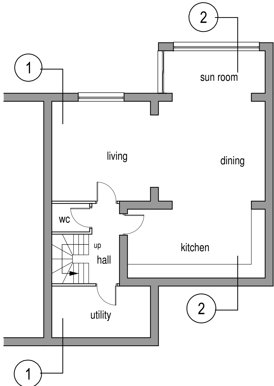
Ground Floor (1:100)
