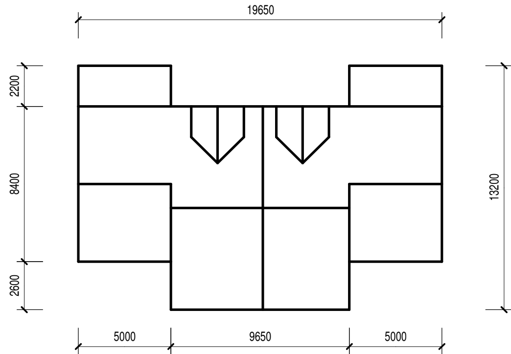
A3 roof plan (1:200)
