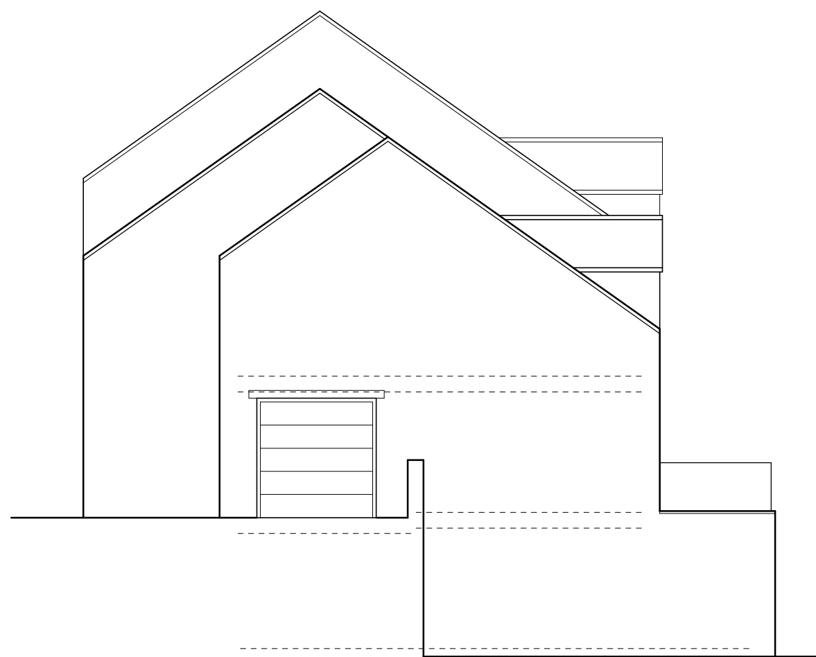
Side elevation (1:100)
