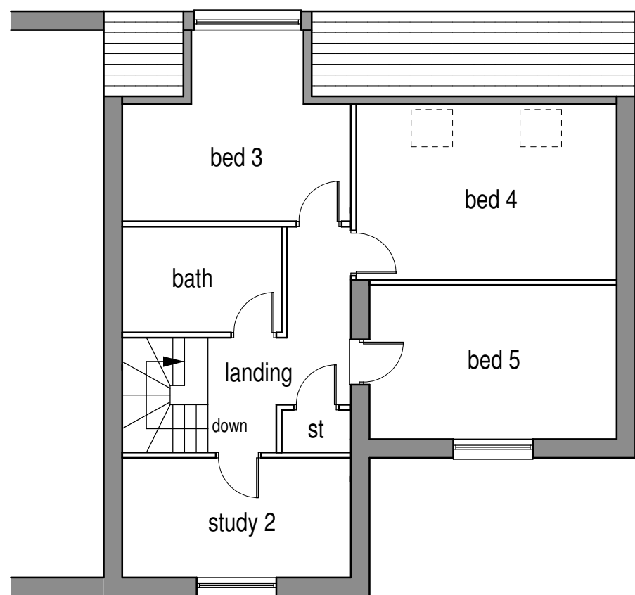
Second Floor (1:100)
