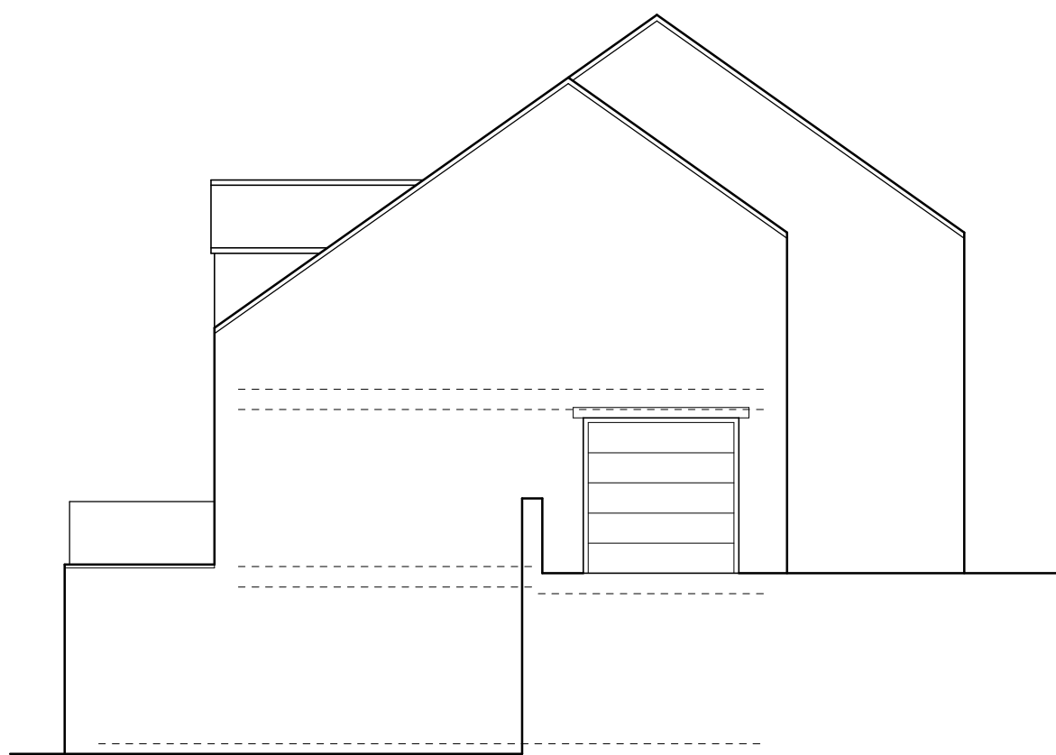
Side elevation (1:100)
