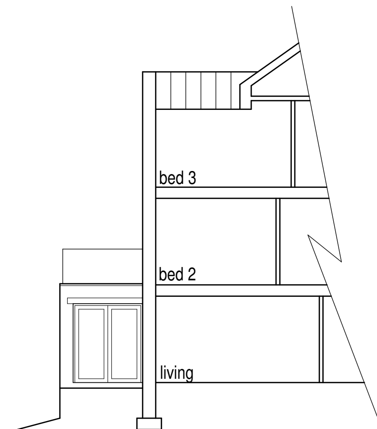
Sectional elevation (1:100)
