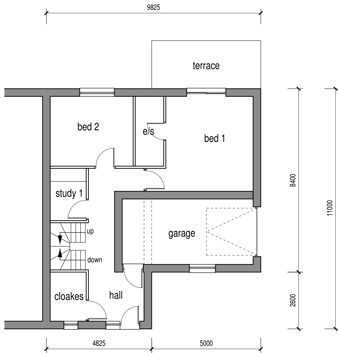
First Floor (1:100)
