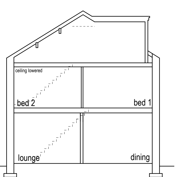
Existing cross section (1:100)
