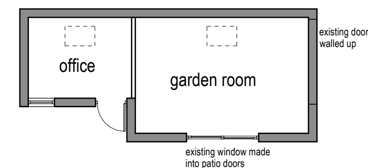
Proposed layout (1:100)
