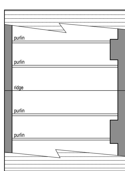
Existing roof layout (1:100)
