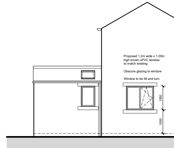
Side Elevation as proposed
