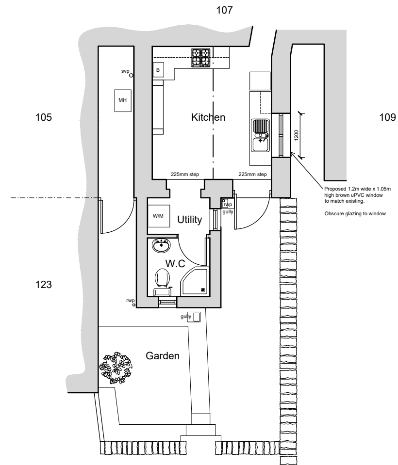
Ground Floor Plan as proposed
