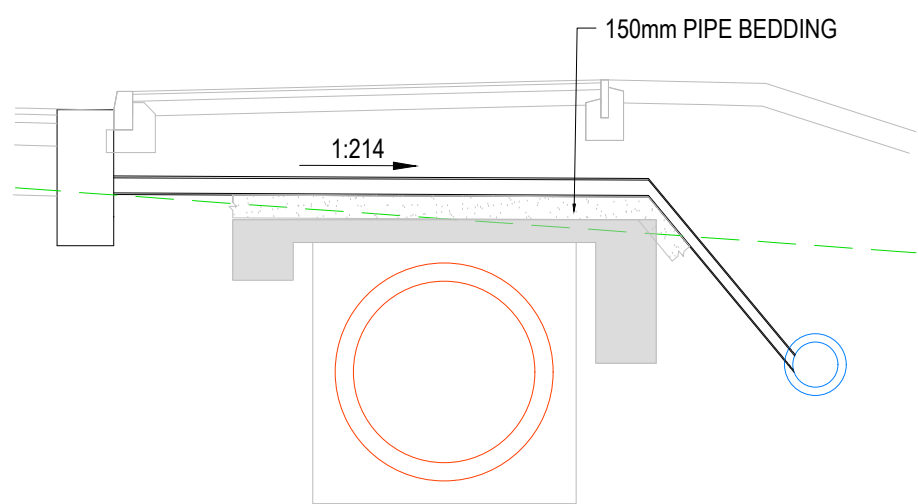
GULLY SECTION 4 (SCALE 1:20)
