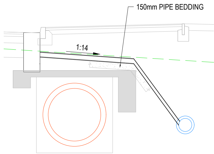
GULLY SECTION 2 (SCALE 1:50)
