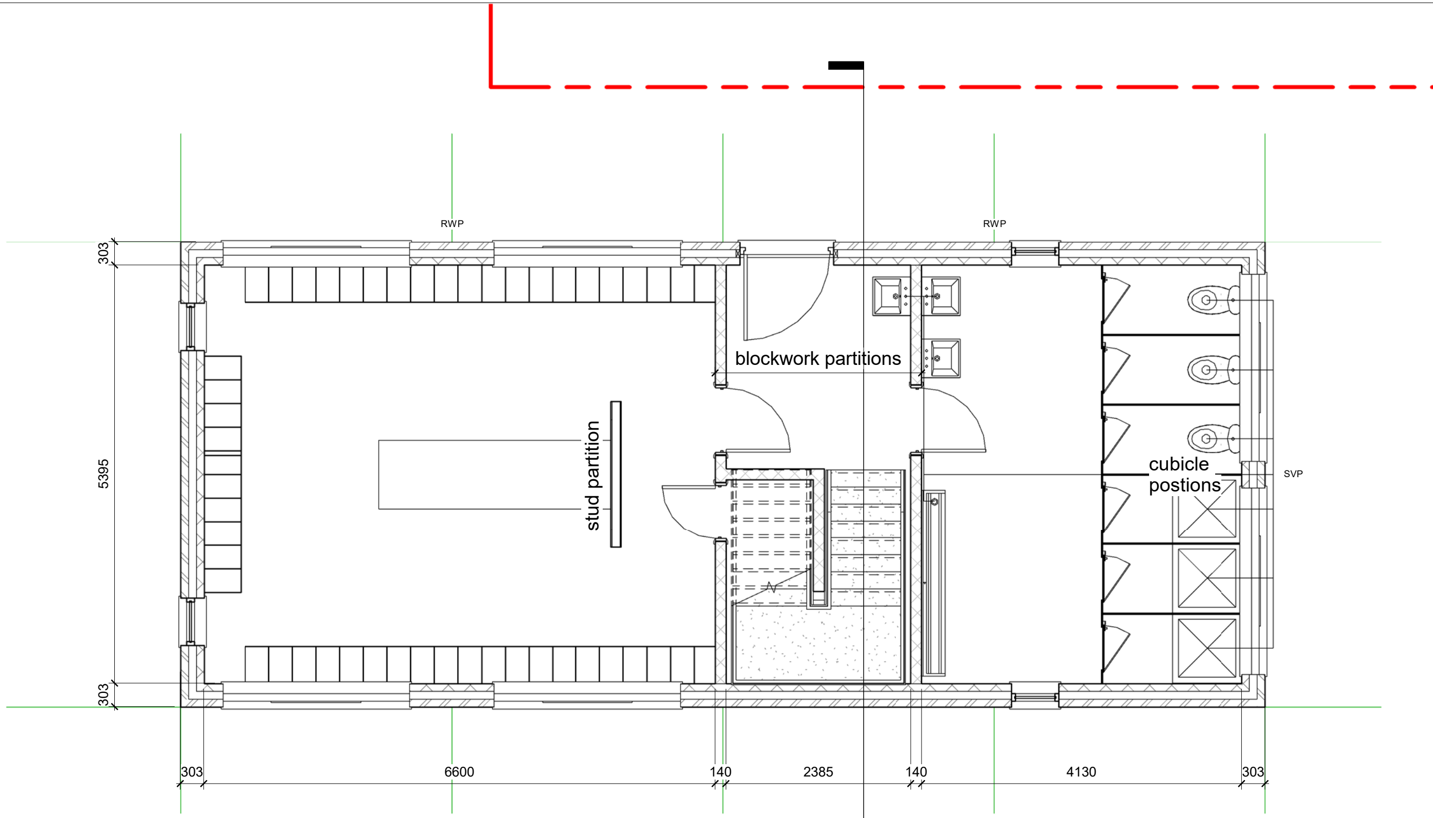
1 11 Grd Floor Detail 1 : 50
