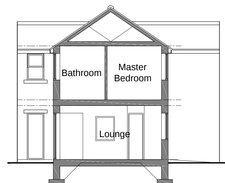
North Elevation / Section A-A - Existing
