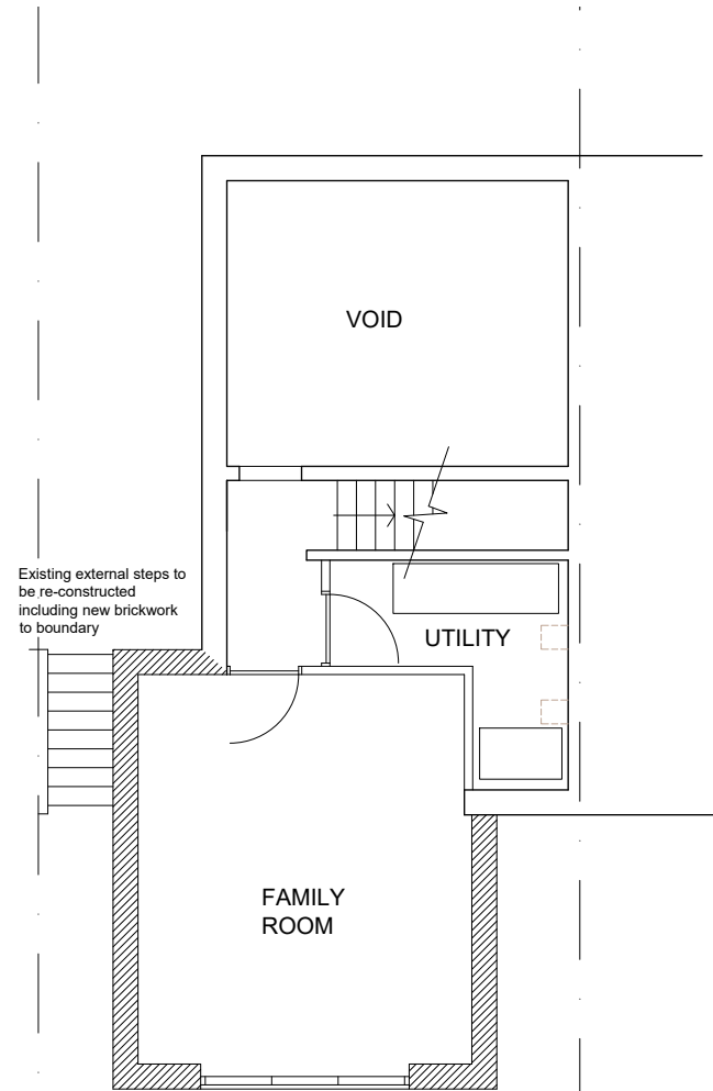
LOWER GROUND FLOOR PROPOSED PLANS 1:100 scale
